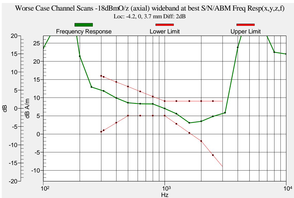
Figure 14: Frequency Response CDMA Cell (-18dbmO) – Channel 384
