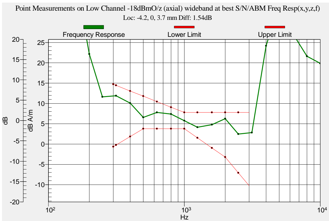
Figure 13: Frequency Response CDMA Cell (-18dbmO) – Channel 1013
