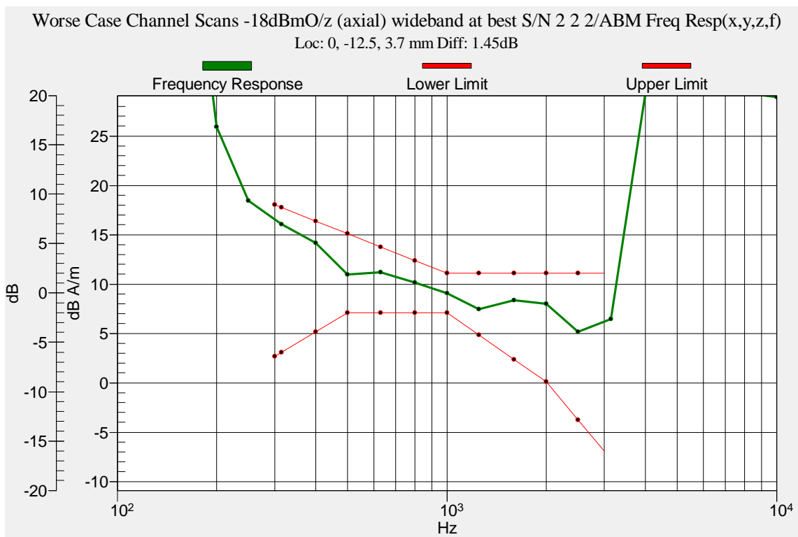
Figure 17: Frequency Response CDMA PCS (-18dbmO) – Channel 600
