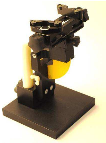
Figure 9: Device Holder
