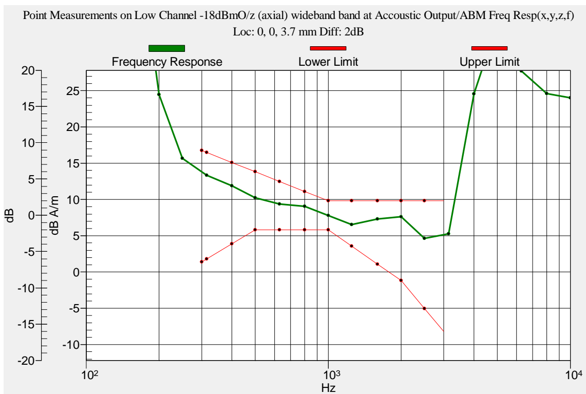
Figure 16: Frequency Response CDMA PCS (-18dbmO) – Channel 25
