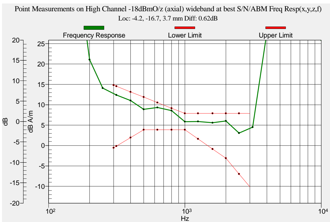
Figure 18: Frequency Response CDMA PCS (-18dbmO) – Channel 1175
