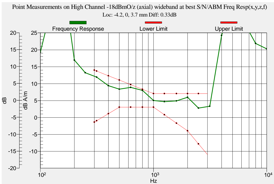
Figure 15: Frequency Response CDMA Cell (-18dbmO) – Channel 777
