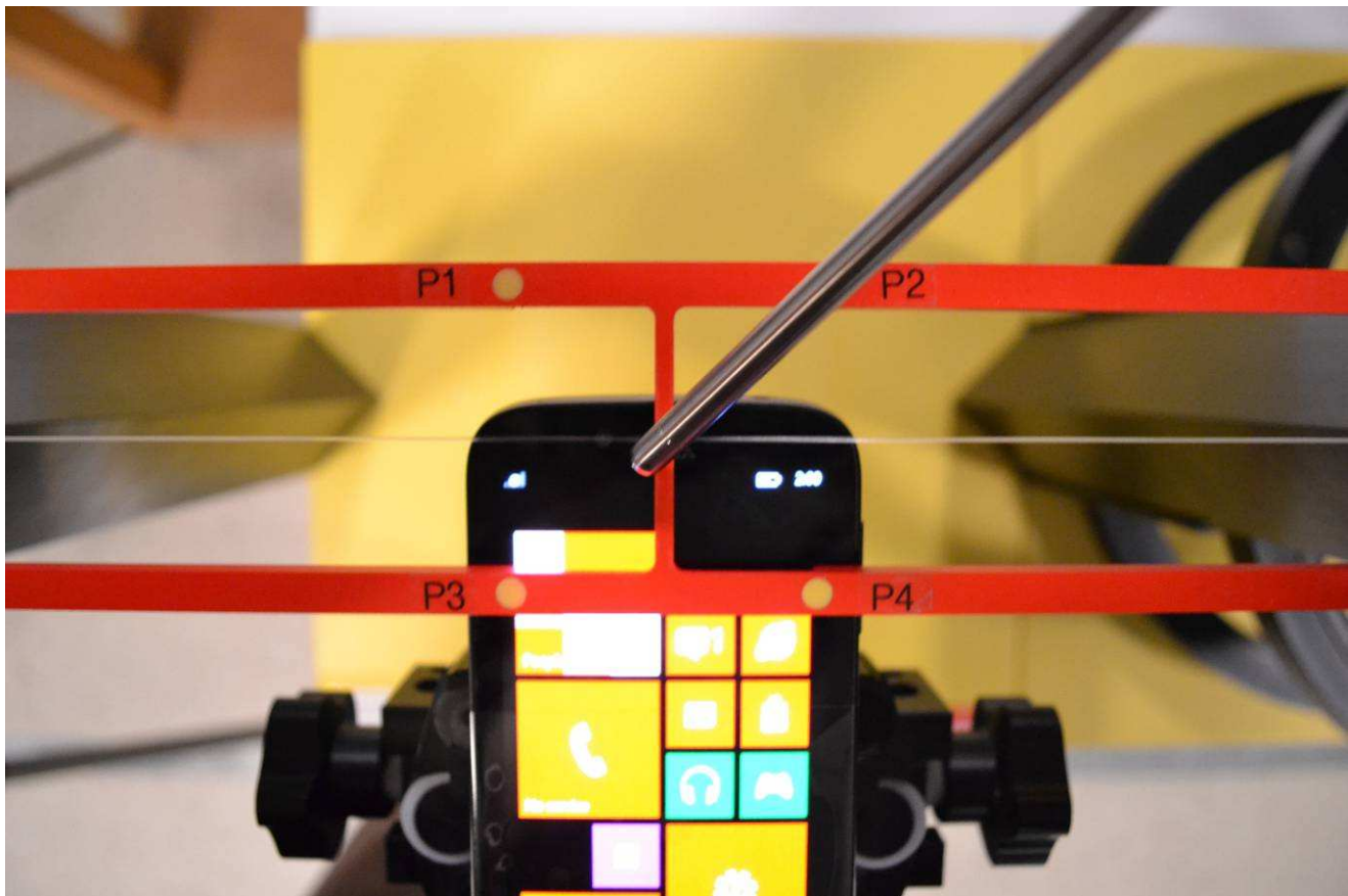
Figure 4: T-Coil Setup Photograph Showing EUT Centered on Test Arch
