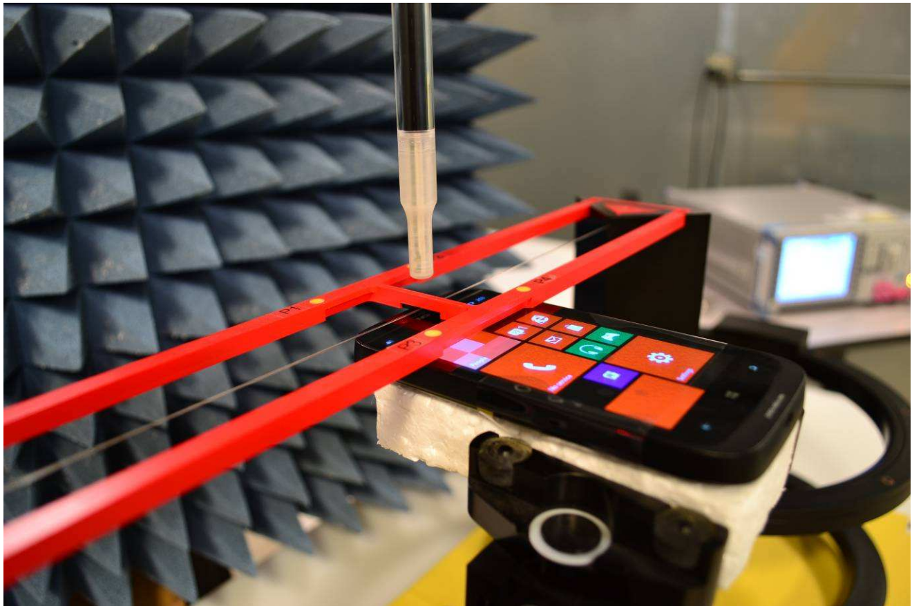
Figure 3: Test Setup Photograph – Near Field Emissions Test
