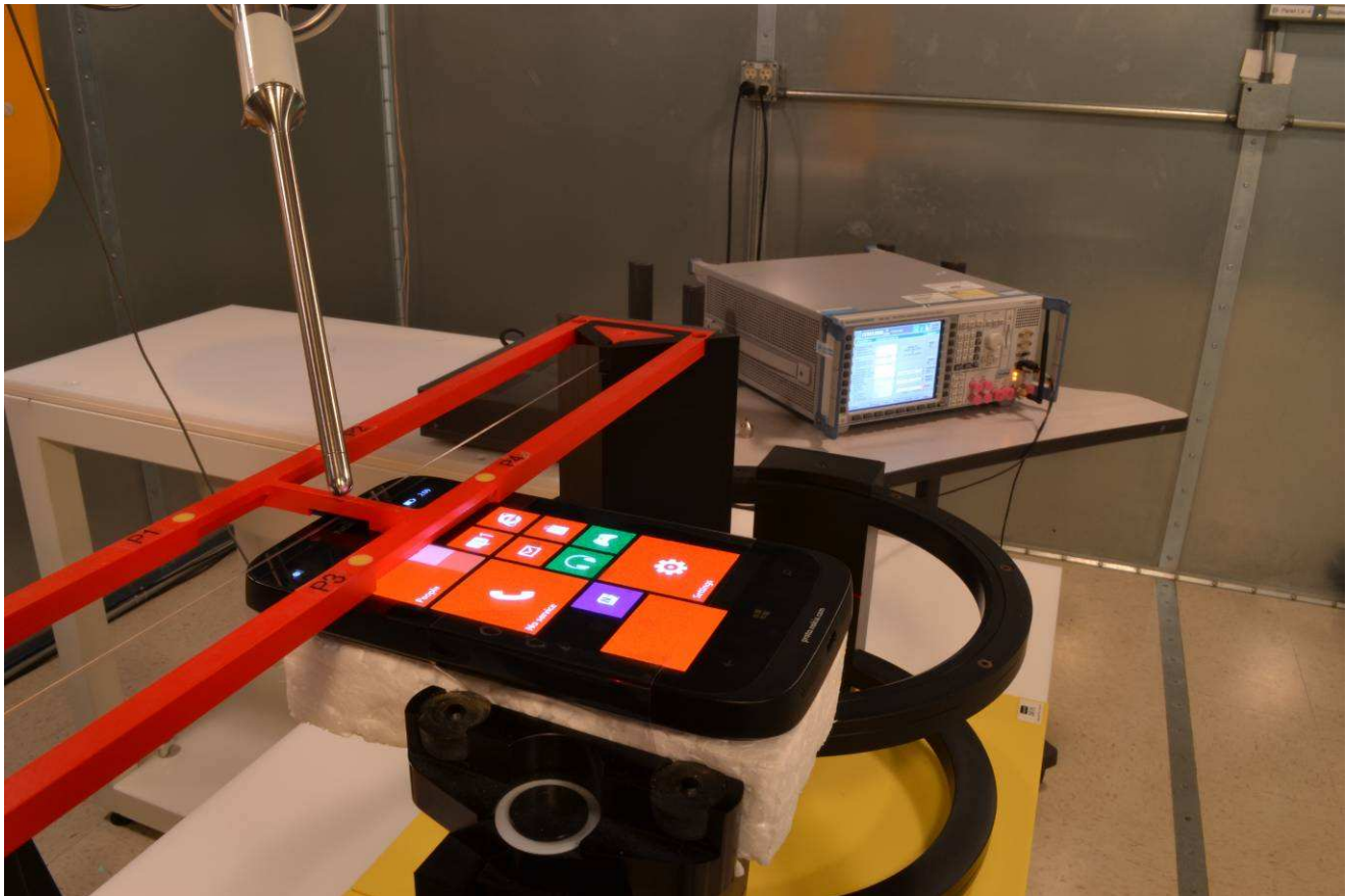
Figure 5: T-Coil Test Setup Photograph
