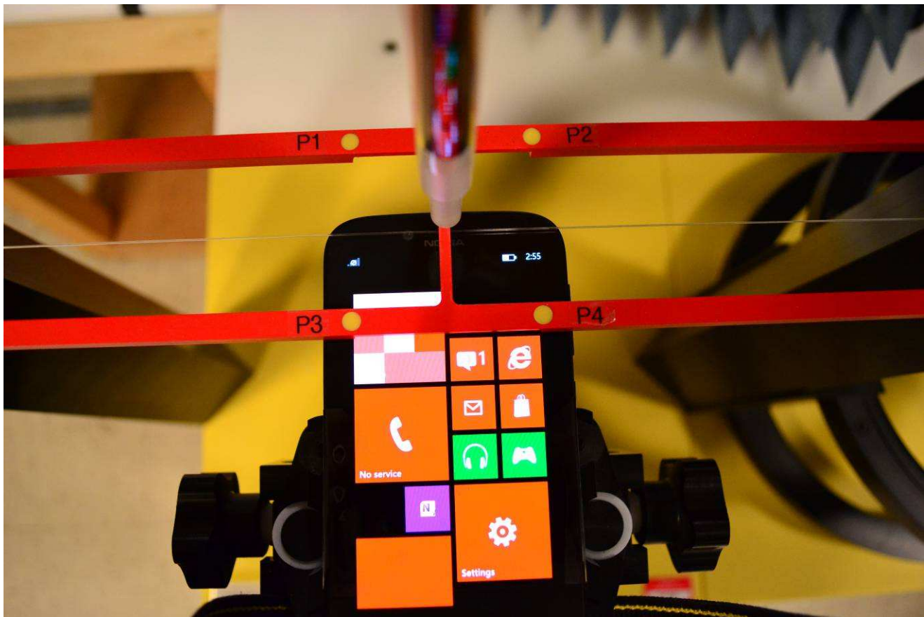
Figure 2: Setup Photograph Showing EUT Centered on Test Arch for RF Emissions Scan
