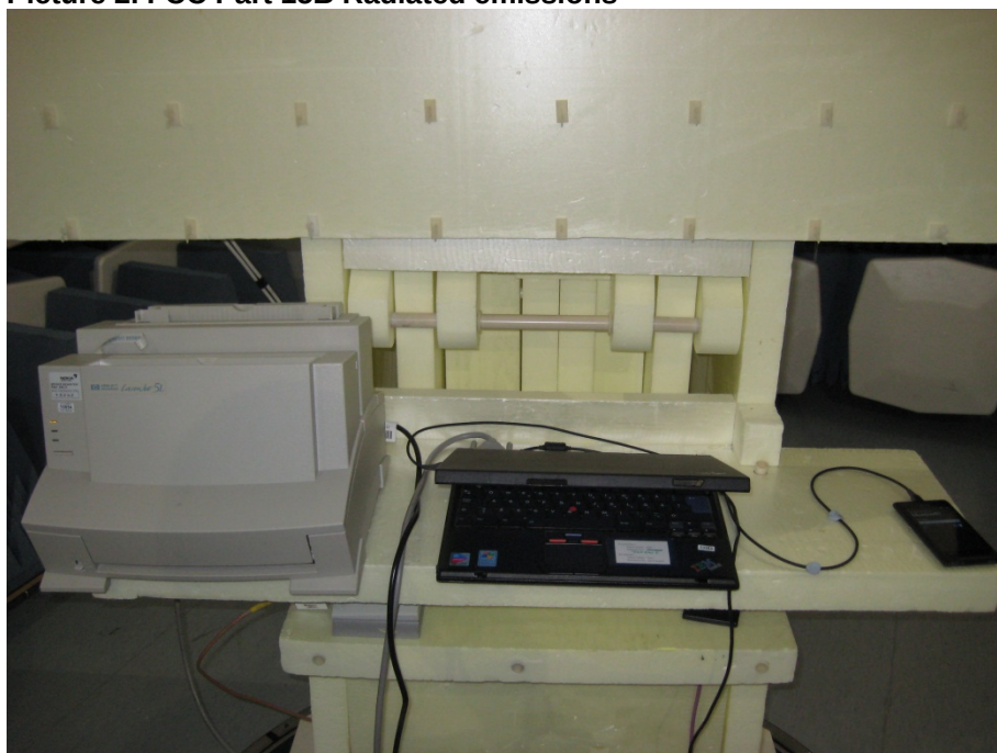
Picture 2. FCC Part 15B Radiated emissions
