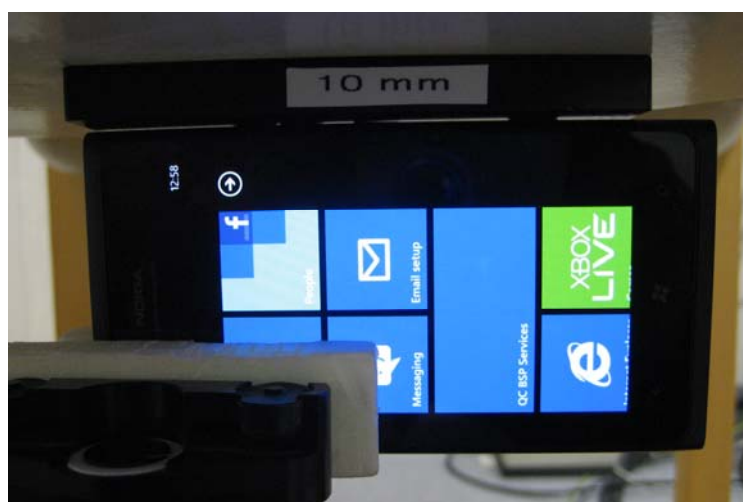
Photo of the device positioned for WR mode measurement – right edge facing phantom. The spacer was removed before the start of the measurements.
