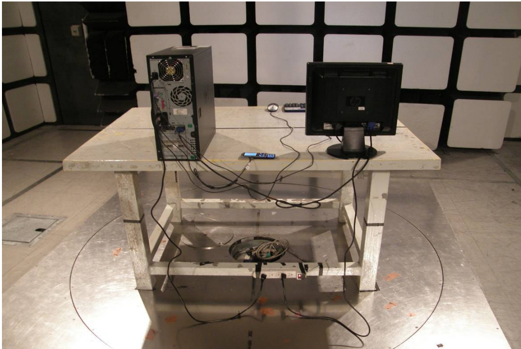
Radiated Emission Test Setup Photo (Data Link Mode)
