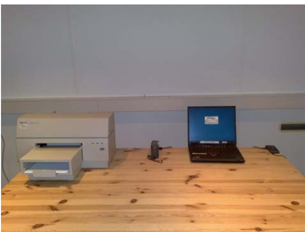
Picture 5 AC powerline conducted emission measurement Bluetooth TX / WLAN TX / FM TX+ Computer peripherals
