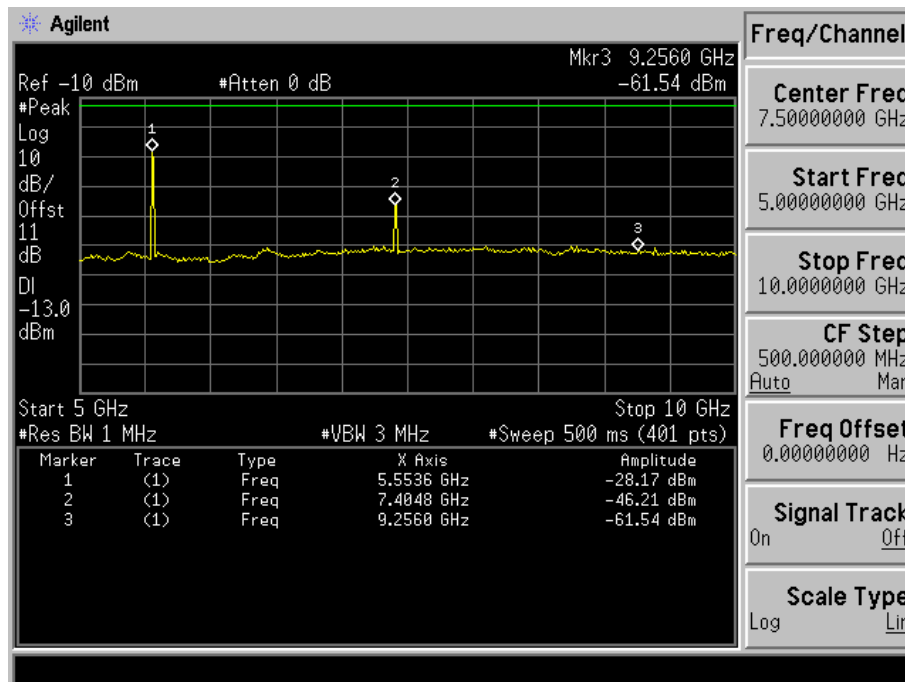
Fig. 5-6(c) Conducted spurious emission for mode 2(Ch. 25).
