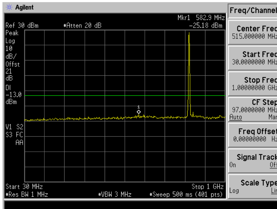
Fig. 5-9(a) Conducted spurious emission for mode 3(Ch. 1013).
