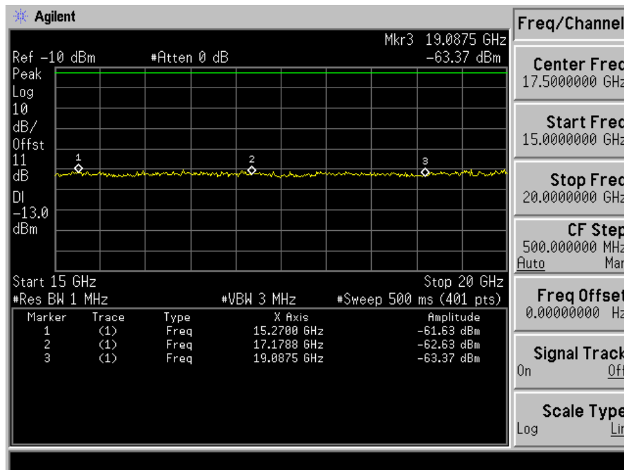
Fig. 5-8(e) Conducted spurious emission for mode 2(Ch. 1175).
