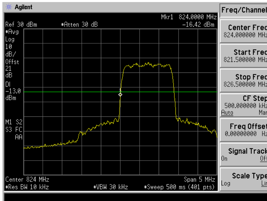
Fig. 4-14 Band edge measurements for mode 3(Ch. 1013).
