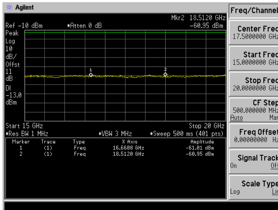
Fig. 5-18(e) Conducted spurious emission for mode 2(Ch. 25).
