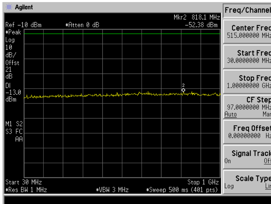
Fig. 5-19(a) Conducted spurious emission for mode 2(Ch. 600).
