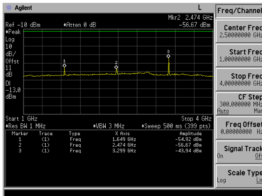
Fig. 5-9(b) Conducted spurious emission for mode 3(Ch. 1013).
