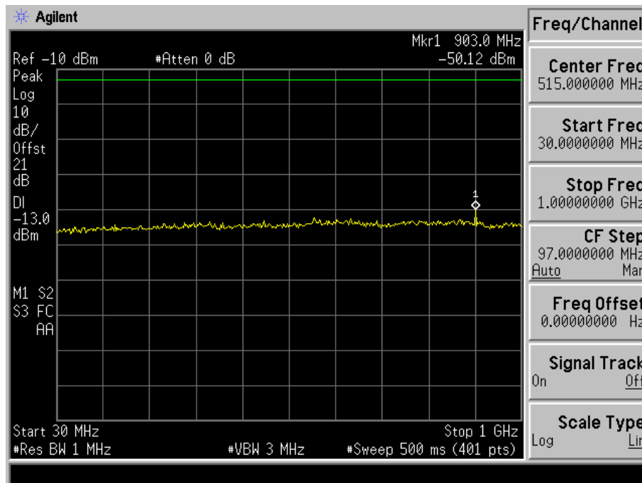
Fig. 5-13(a) Conducted spurious emission for mode 4(Ch. 600).
