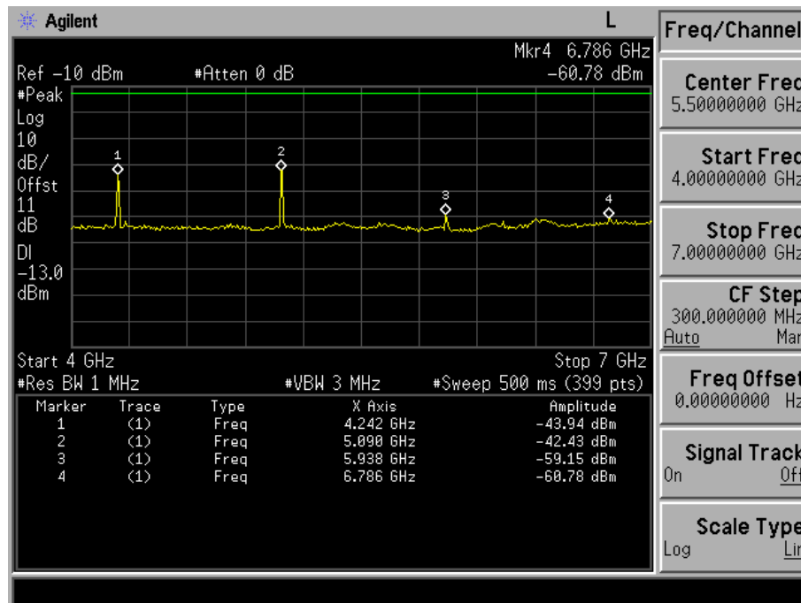
Fig. 5-23(c) Conducted spurious emission for mode 3(Ch. 777).
