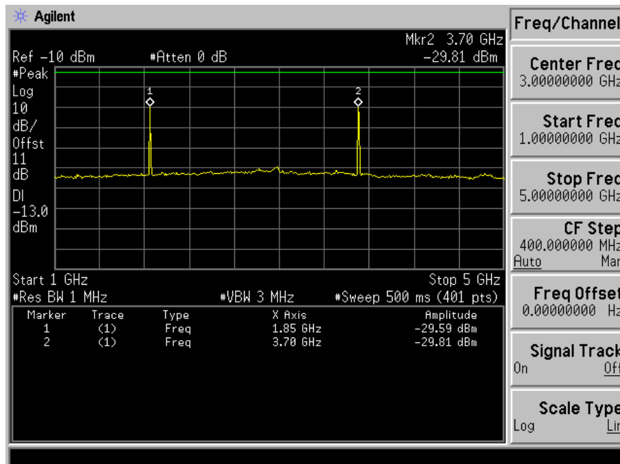
Fig. 5-6(b) Conducted spurious emission for mode 2(Ch. 25).
