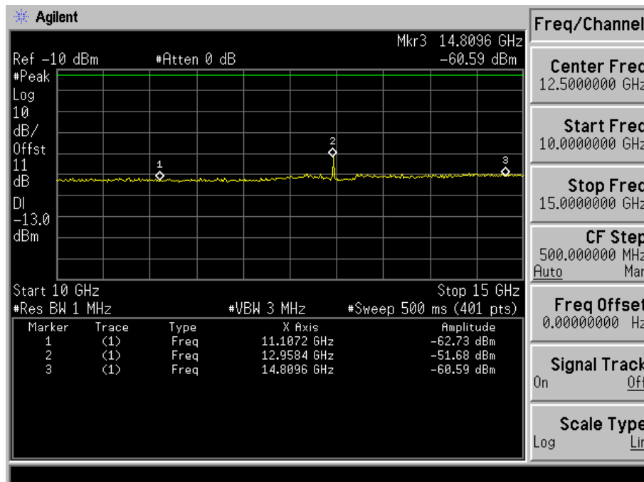
Fig. 5-24(d) Conducted spurious emission for mode 4(Ch. 25).
