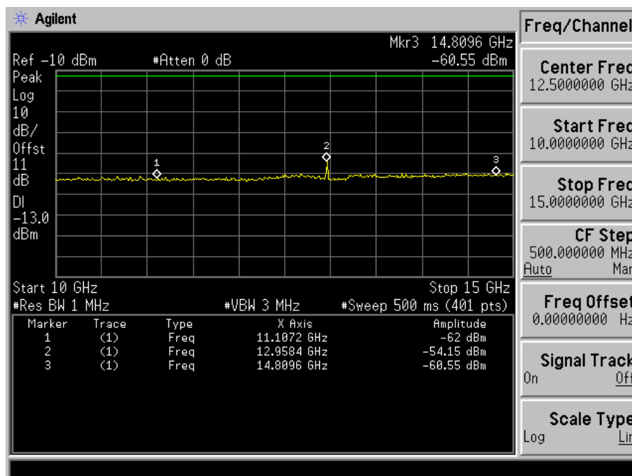
Fig. 5-18(d) Conducted spurious emission for mode 2(Ch. 25).
