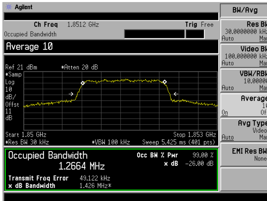
Fig. 3-5 Occupied Bandwidth for mode 2(Ch. 25).
