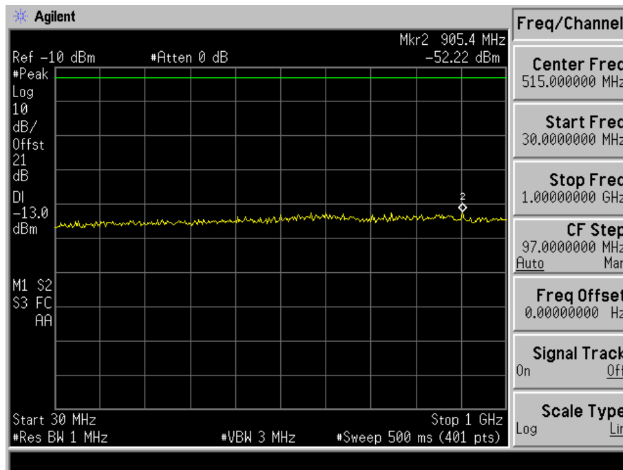
Fig. 5-25(a) Conducted spurious emission for mode 4(Ch. 600).
