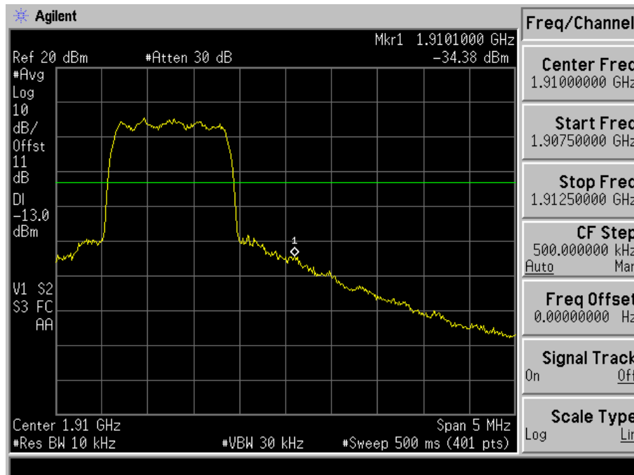
Fig. 4-9 Band edge measurements for mode 4(Ch. 1175).
