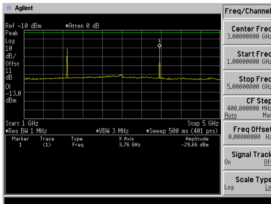
Fig. 5-19(b) Conducted spurious emission for mode 2(Ch. 600).
