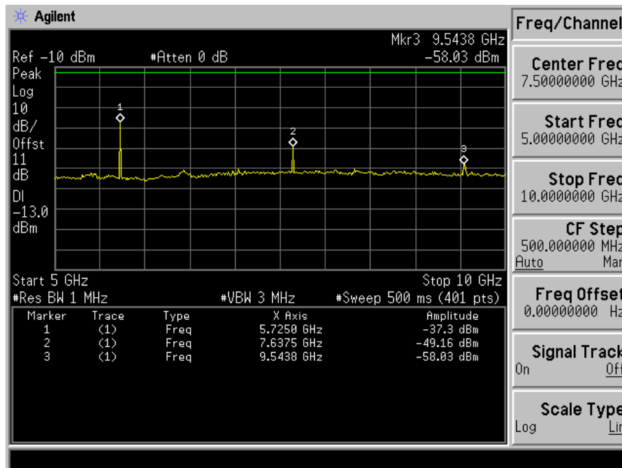
Fig. 5-14(c) Conducted spurious emission for mode 4(Ch. 1175).
