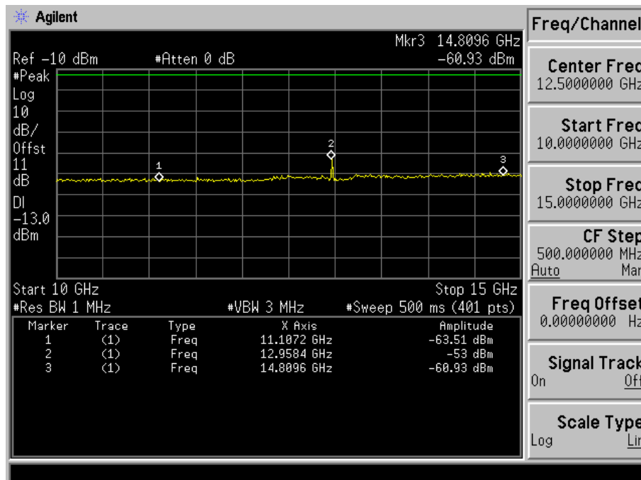
Fig. 5-6(d) Conducted spurious emission for mode 2(Ch. 25).
