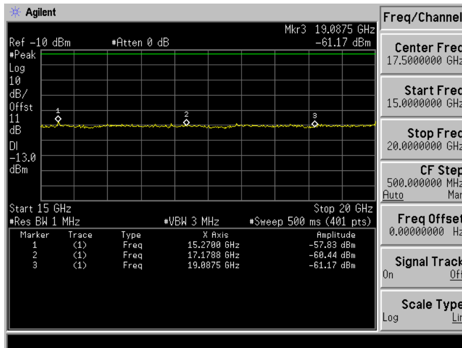
Fig. 5-26(e) Conducted spurious emission for mode 4(Ch. 1175).
