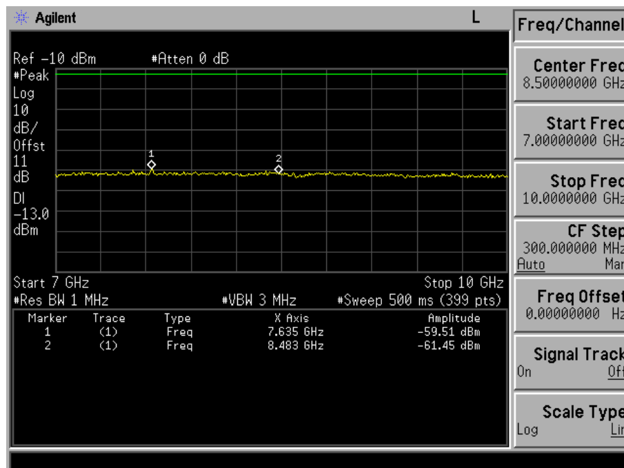
Fig. 5-17(d) Conducted spurious emission for mode 1(Ch. 777).
