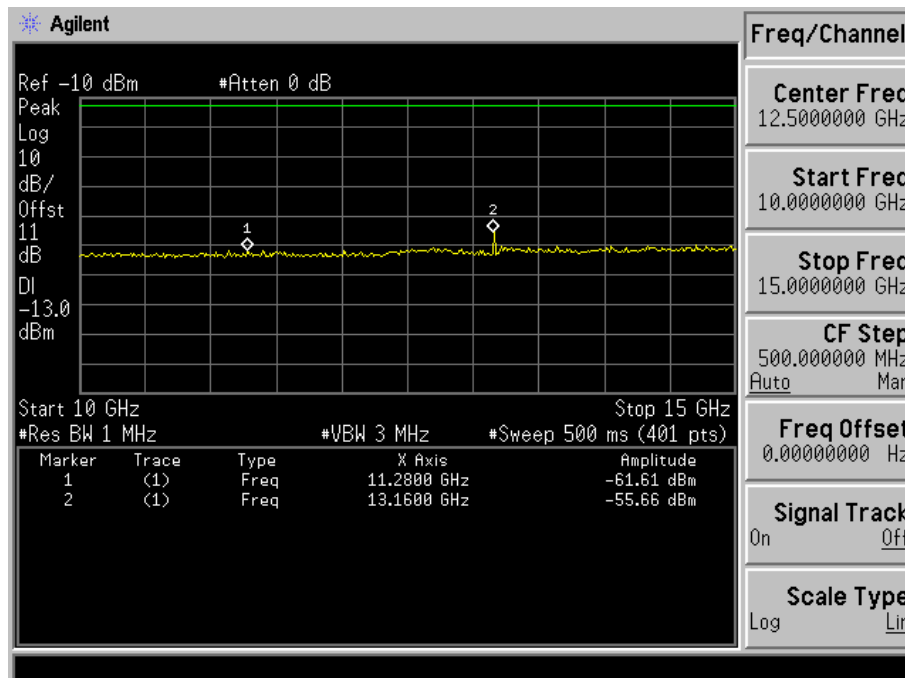
Fig. 5-19(d) Conducted spurious emission for mode 2(Ch. 600).
