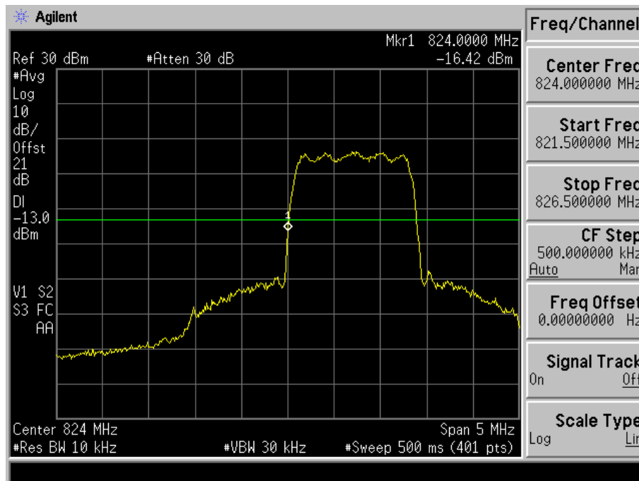
Fig. 4-6 Band edge measurements for mode 3(Ch. 1013).
