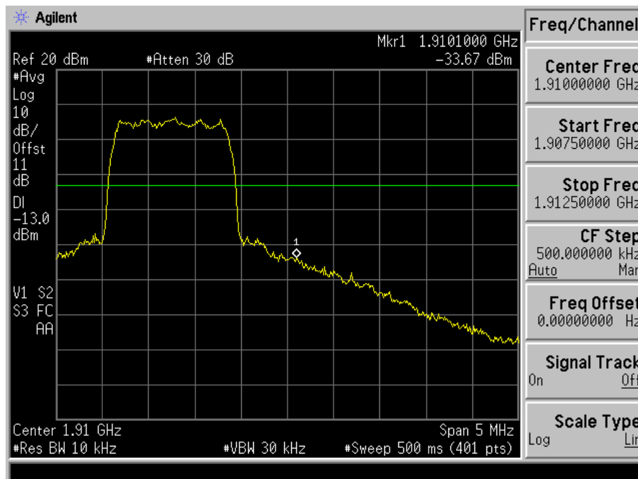
Fig. 4-13 Band edge measurements for mode 2(Ch. 1175).
