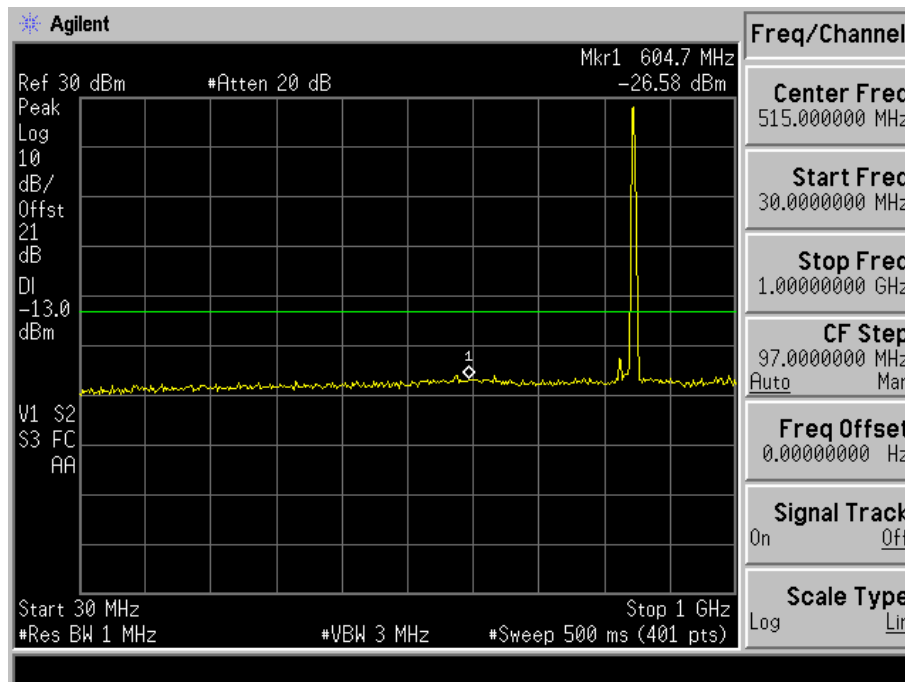
Fig. 5-11(a) Conducted spurious emission for mode 3(Ch. 777).
