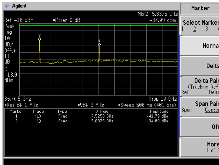
Fig. 5-13(c) Conducted spurious emission for mode 4(Ch. 600).
