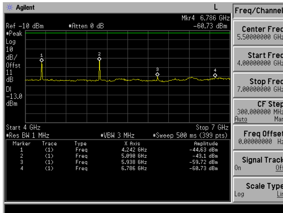
Fig. 5-17(c) Conducted spurious emission for mode 1(Ch. 777).
