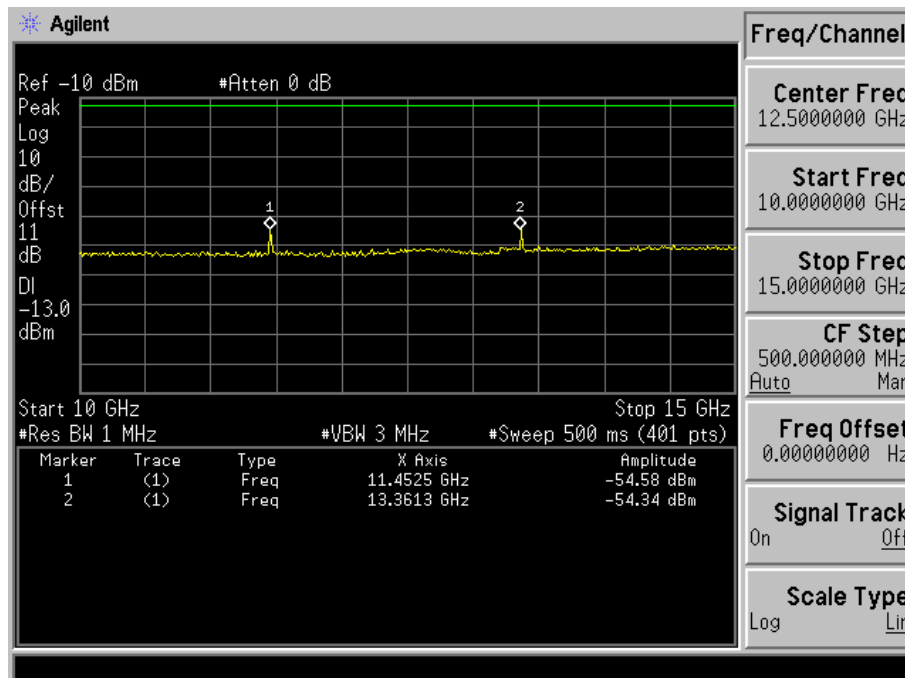
Fig. 5-14(d) Conducted spurious emission for mode 4(Ch. 1175).
