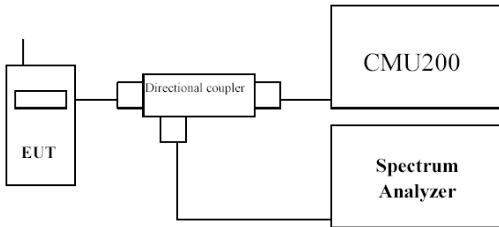
Fig. 3-1 Test setup.
