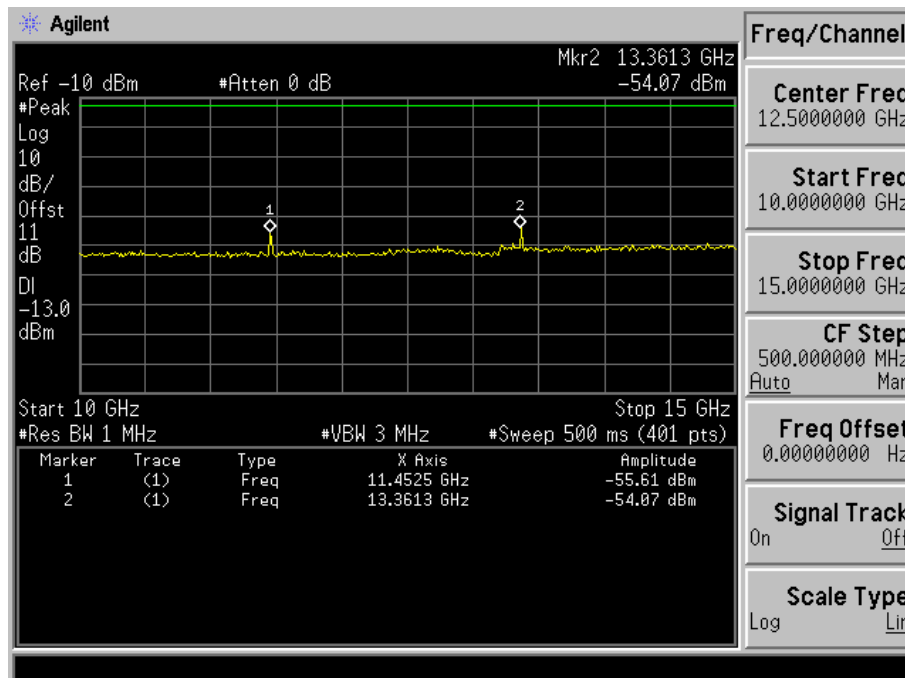
Fig. 5-26(d) Conducted spurious emission for mode 4(Ch. 1175).
