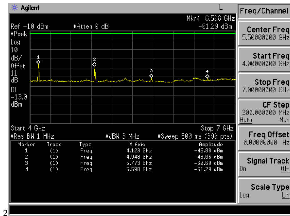
Fig. 5-21(c) Conducted spurious emission for mode 3(Ch. 1013).
