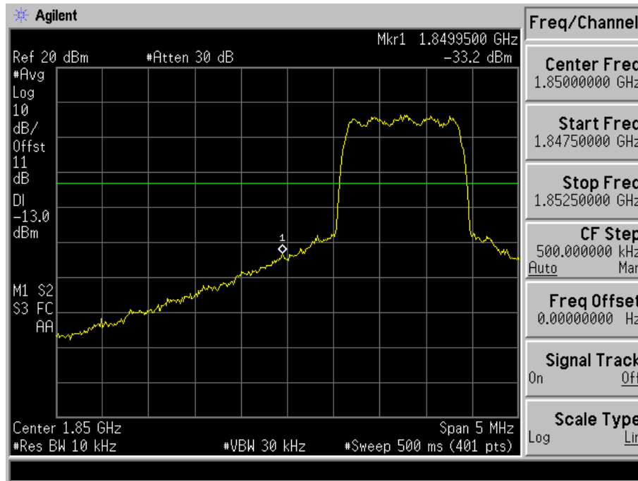
Fig. 4-12 Band edge measurements for mode 2(Ch. 25).
