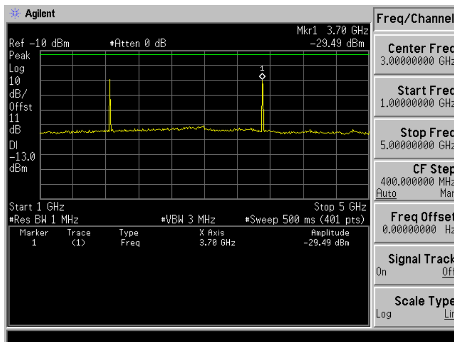
Fig. 5-18(b) Conducted spurious emission for mode 2(Ch. 25).
