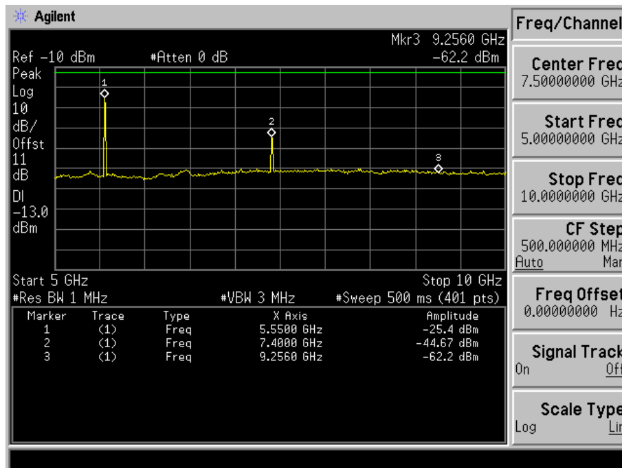
Fig. 5-12(c) Conducted spurious emission for mode 4(Ch. 25).
