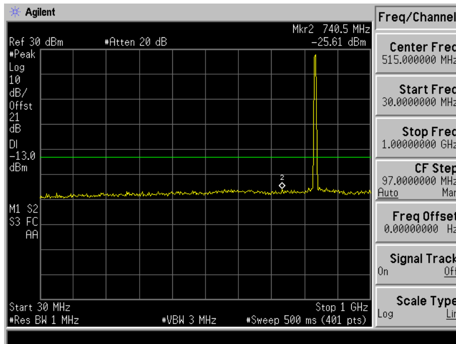
Fig. 5-21(a) Conducted spurious emission for mode 3(Ch. 1013).
