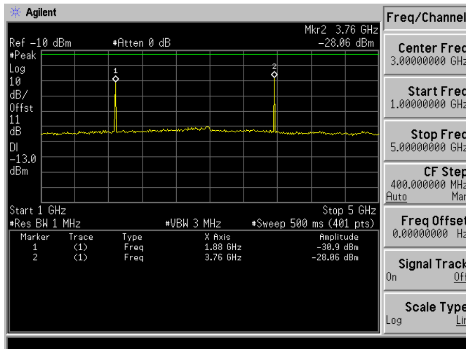
Fig. 5-25(b) Conducted spurious emission for mode 4(Ch. 600).
