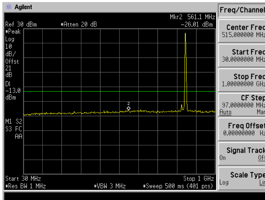
Fig. 5-16(a) Conducted spurious emission for mode 1(Ch. 384).
