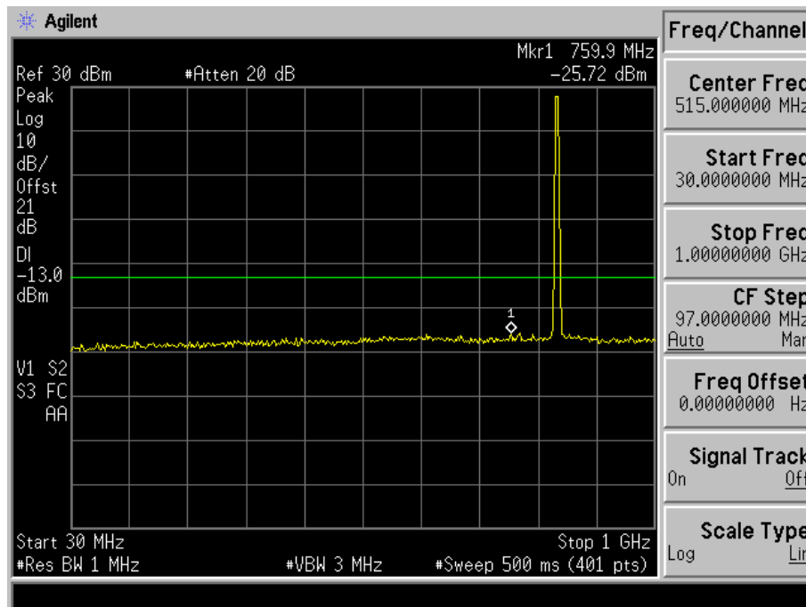
Fig. 5-10(a) Conducted spurious emission for mode 3(Ch. 384).
