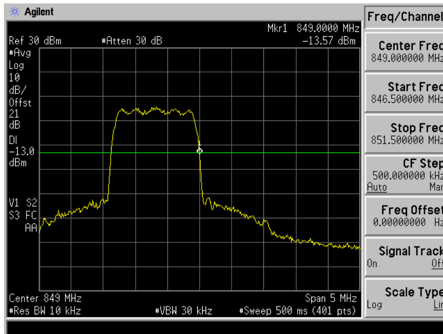
Fig. 4-7 Band edge measurements for mode 3(Ch. 777).
