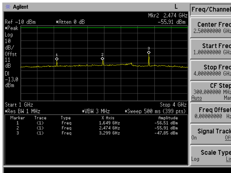
Fig. 5-15(b) Conducted spurious emission for mode 1(Ch. 1013).
