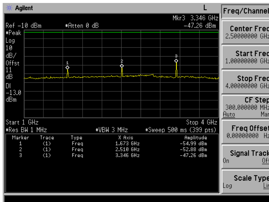
Fig. 5-22(b) Conducted spurious emission for mode 3(Ch. 384).
