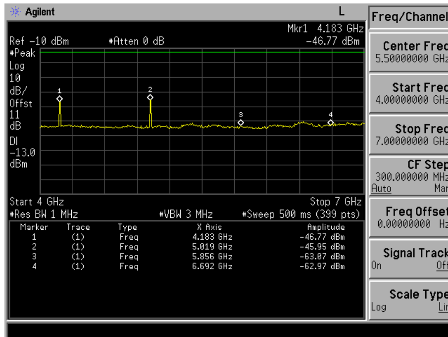
Fig. 5-16(c) Conducted spurious emission for mode 1(Ch. 384).
