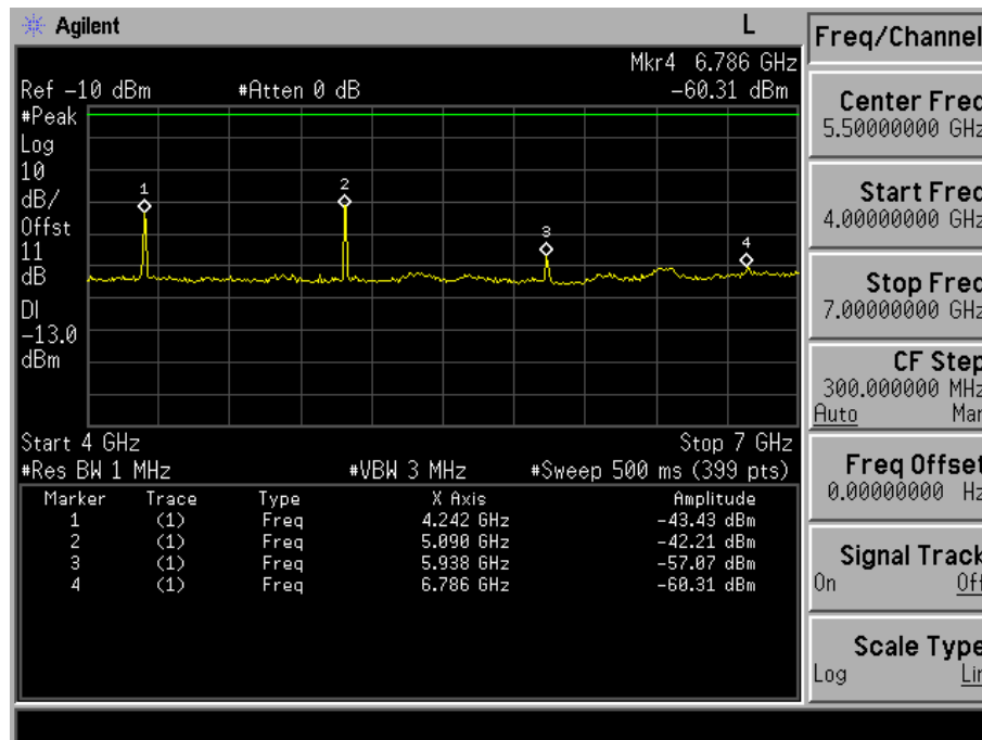
Fig. 5-11(c) Conducted spurious emission for mode 3(Ch. 777).
