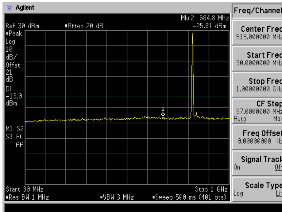
Fig. 5-23(a) Conducted spurious emission for mode 3(Ch. 777).
