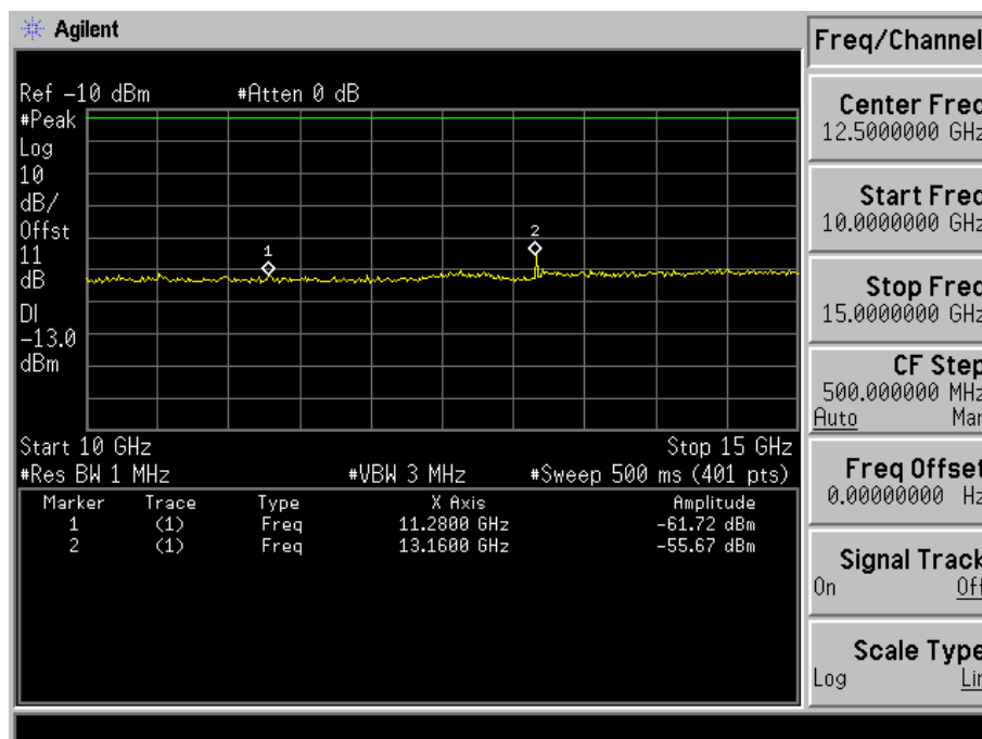
Fig. 5-7(d) Conducted spurious emission for mode 2(Ch. 600).
