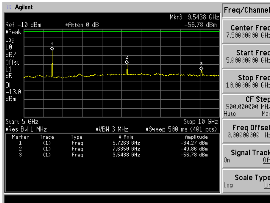
Fig. 5-26(c) Conducted spurious emission for mode 4(Ch. 1175).
