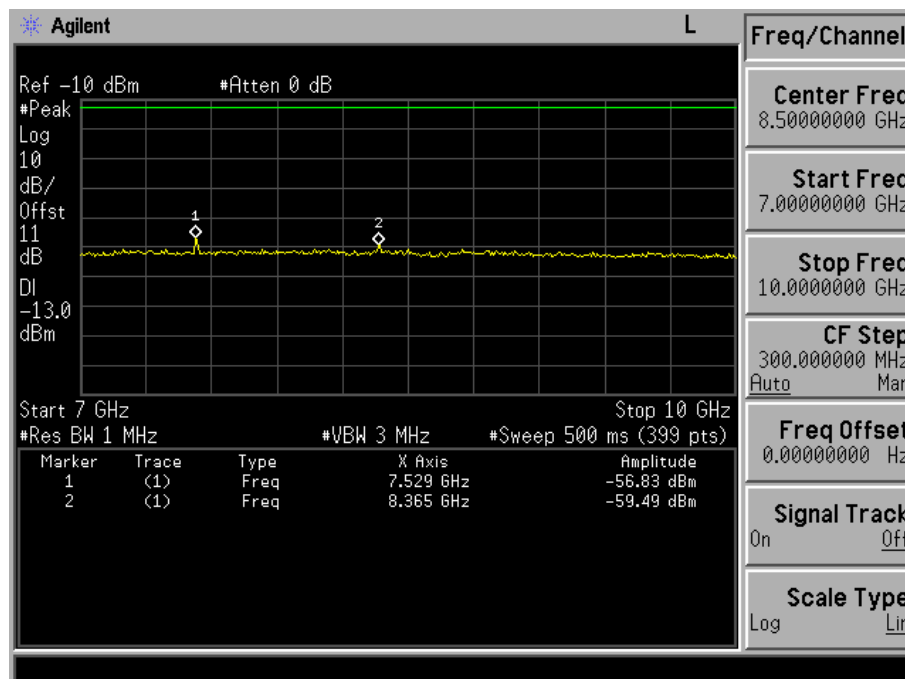
Fig. 5-10(d) Conducted spurious emission for mode 3(Ch. 384).
