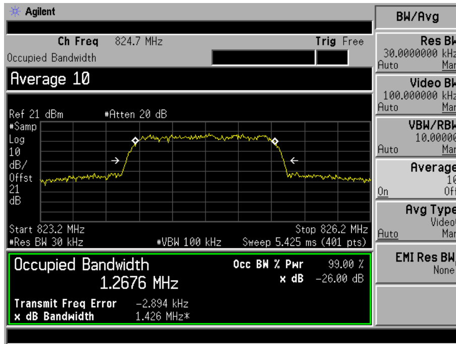
Fig. 3-8 Occupied Bandwidth for mode 3(Ch. 1013).
