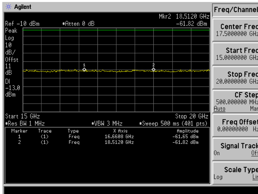
Fig. 5-12(e) Conducted spurious emission for mode 4(Ch. 25).
