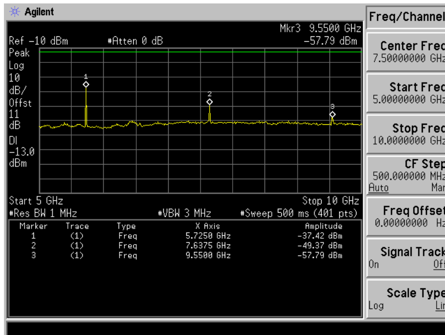
Fig. 5-8(c) Conducted spurious emission for mode 2(Ch. 1175).
