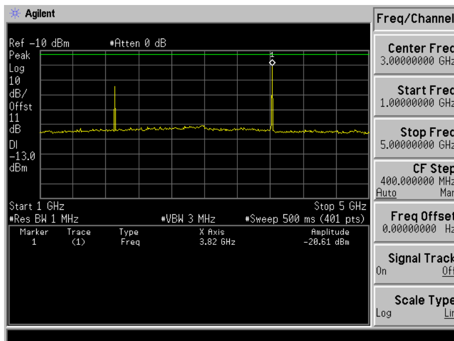
Fig. 5-8(b) Conducted spurious emission for mode 2(Ch. 1175).
