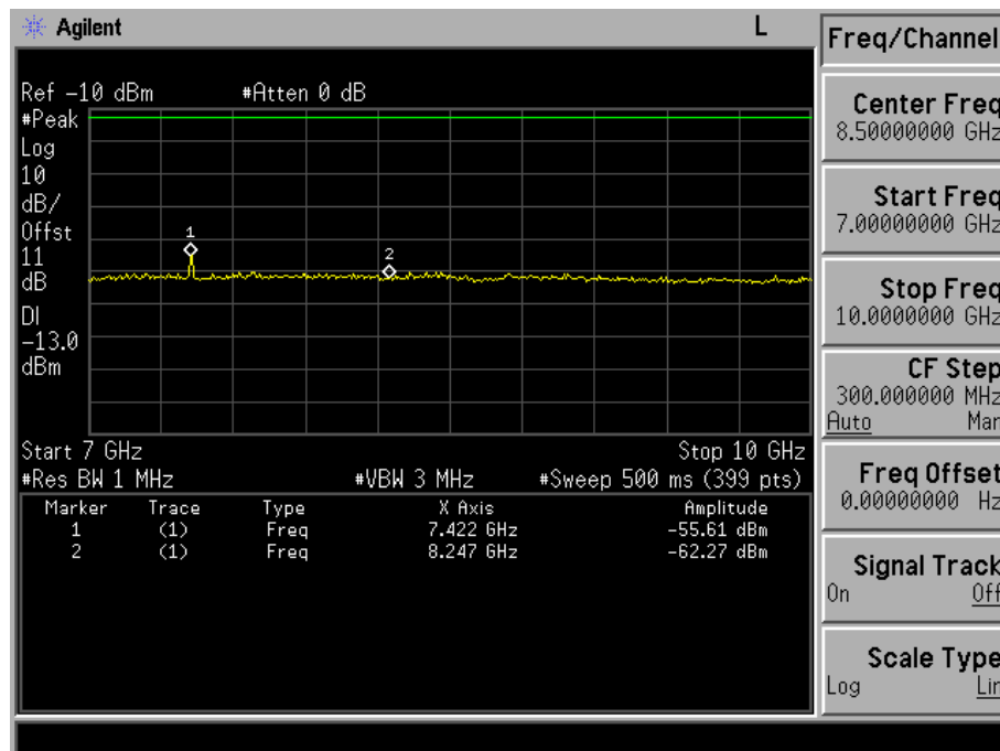
Fig. 5-21(d) Conducted spurious emission for mode 3(Ch. 1013).
