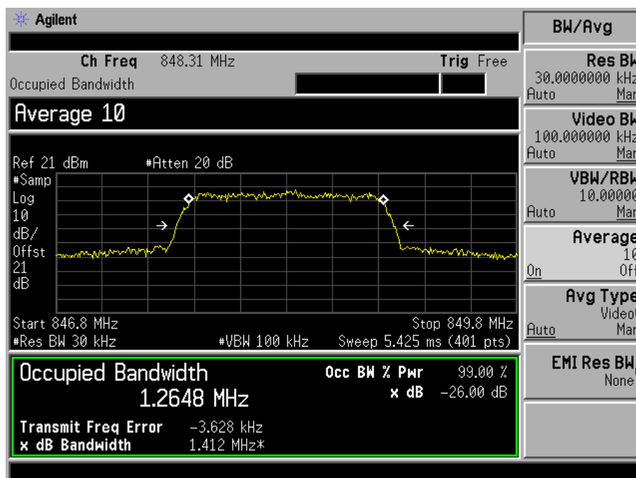
Fig. 3-10 Occupied Bandwidth for mode 3(Ch. 777).
