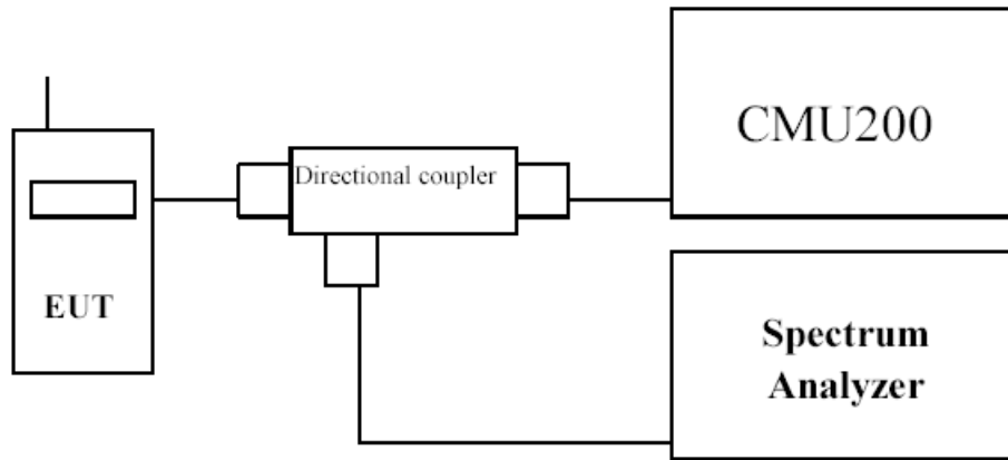
Fig. 5-1 Test setup for conducted spurious measurements.
