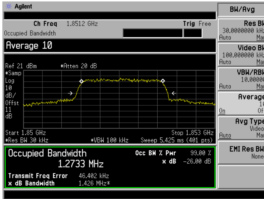
Fig. 3-11 Occupied Bandwidth for mode 4(Ch. 25).
