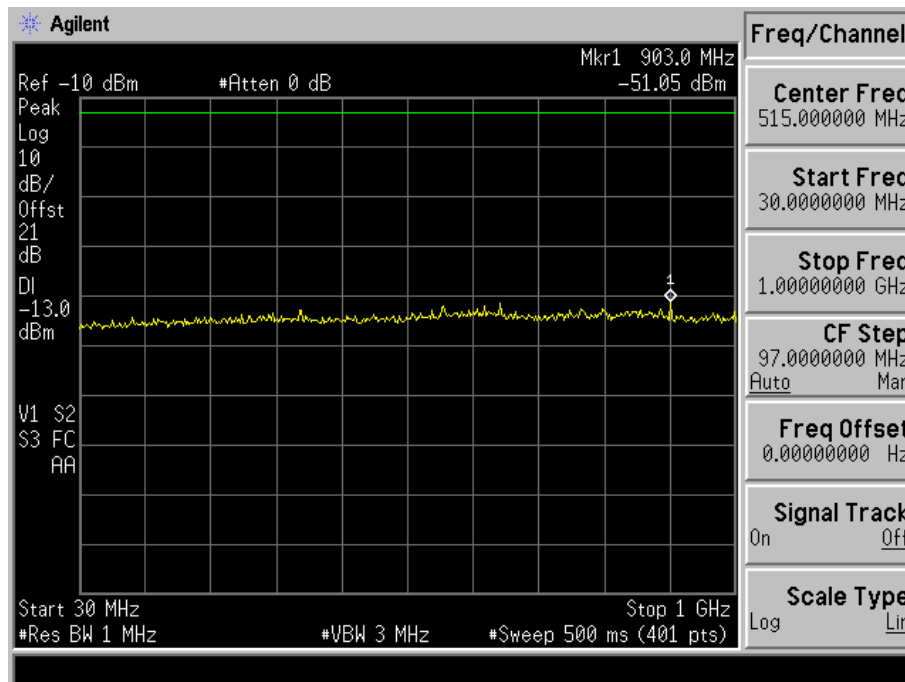
Fig. 5-8(a) Conducted spurious emission for mode 2(Ch. 1175).
