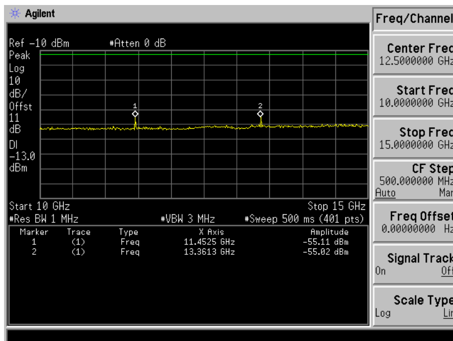
Fig. 5-20(d) Conducted spurious emission for mode 2(Ch. 1175).
