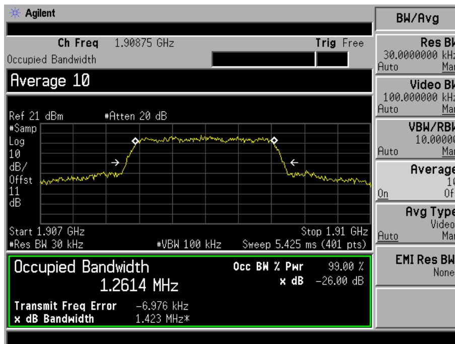
Fig. 3-7 Occupied Bandwidth for mode 2(Ch. 1175).
