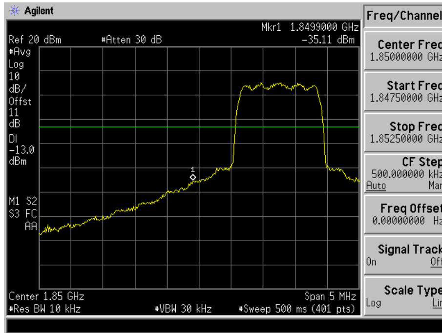
Fig. 4-16 Band edge measurements for mode 4(Ch. 25).
