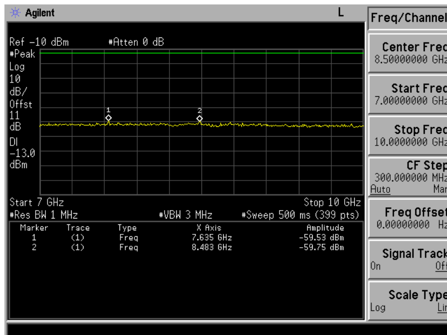
Fig. 5-11(d) Conducted spurious emission for mode 3(Ch. 777).
