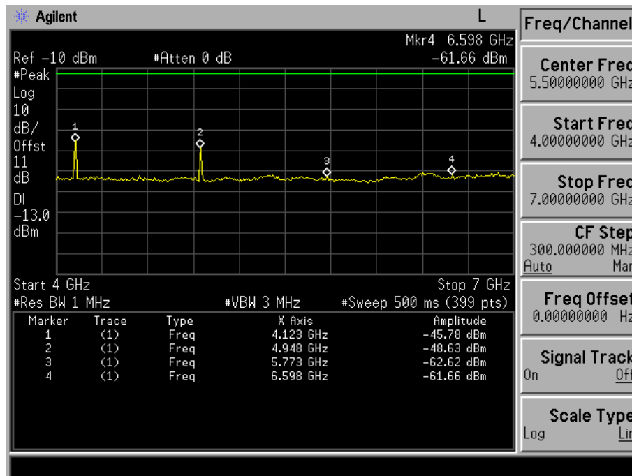
Fig. 5-15(c) Conducted spurious emission for mode 1(Ch. 1013).
