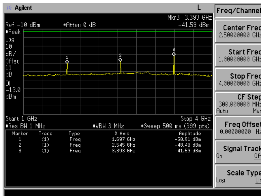
Fig. 5-23(b) Conducted spurious emission for mode 3(Ch. 777).
