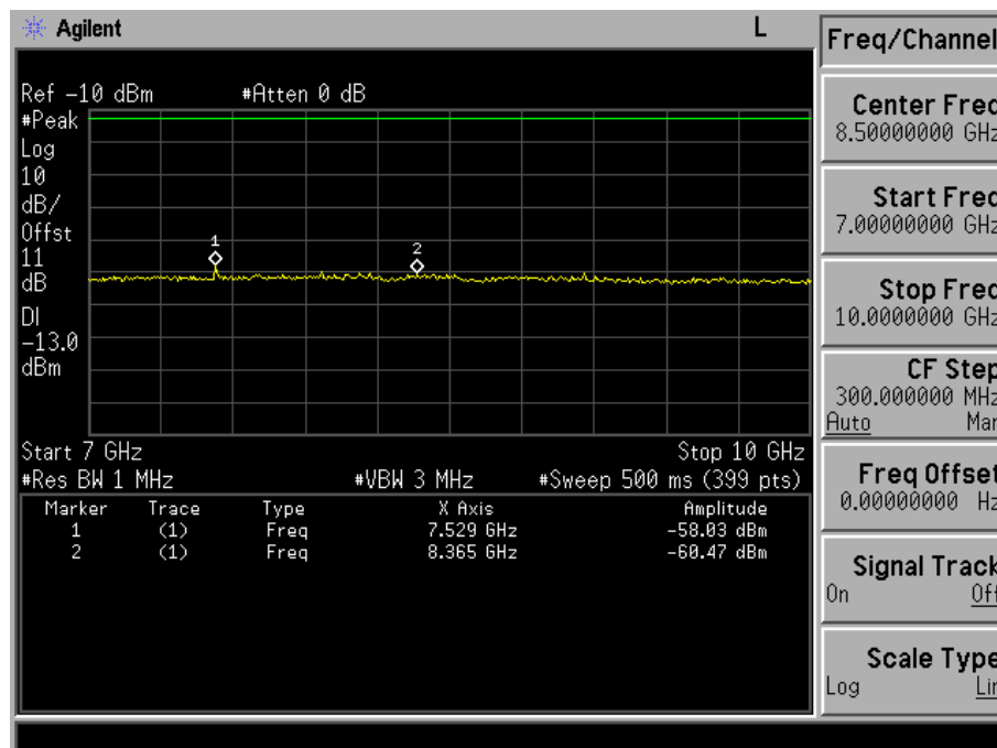
Fig. 5-16(d) Conducted spurious emission for mode 1(Ch. 384).
