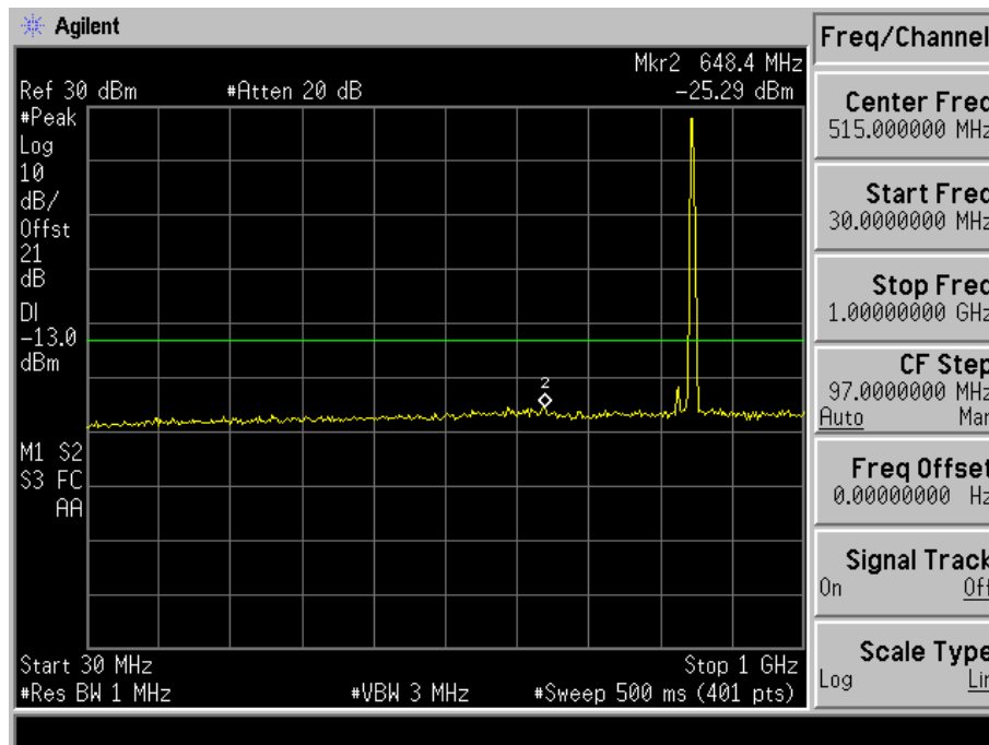
Fig. 5-22(a) Conducted spurious emission for mode 3(Ch. 384).
