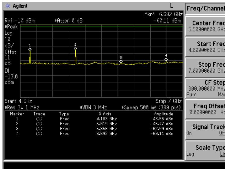
Fig. 5-22(c) Conducted spurious emission for mode 3(Ch. 384).
