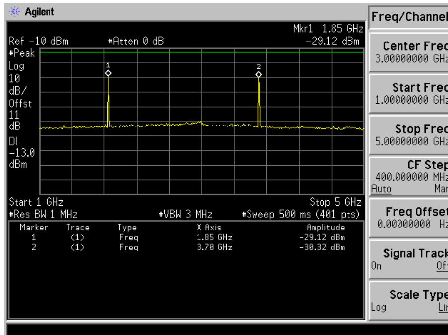
Fig. 5-24(b) Conducted spurious emission for mode 4(Ch. 25).
