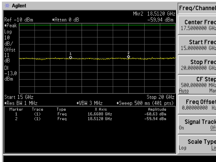
Fig. 5-24(e) Conducted spurious emission for mode 4(Ch. 25).
