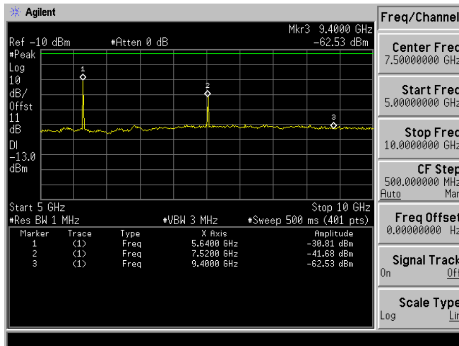
Fig. 5-25(c) Conducted spurious emission for mode 4(Ch. 600).
