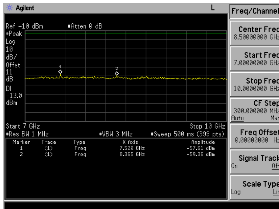
Fig. 5-22(d) Conducted spurious emission for mode 3(Ch. 384).
