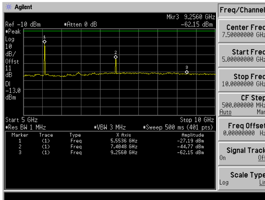
Fig. 5-24(c) Conducted spurious emission for mode 4(Ch. 25).
