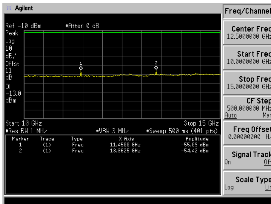
Fig. 5-8(d) Conducted spurious emission for mode 2(Ch. 1175).
