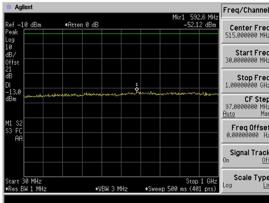
Fig. 5-12(a) Conducted spurious emission for mode 4(Ch. 25).
