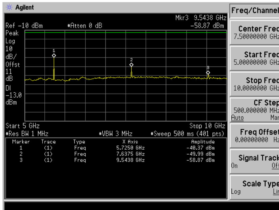
Fig. 5-20(c) Conducted spurious emission for mode 2(Ch. 1175).
