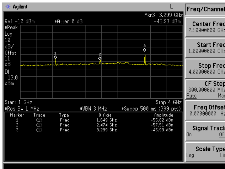
Fig. 5-21(b) Conducted spurious emission for mode 3(Ch. 1013).
