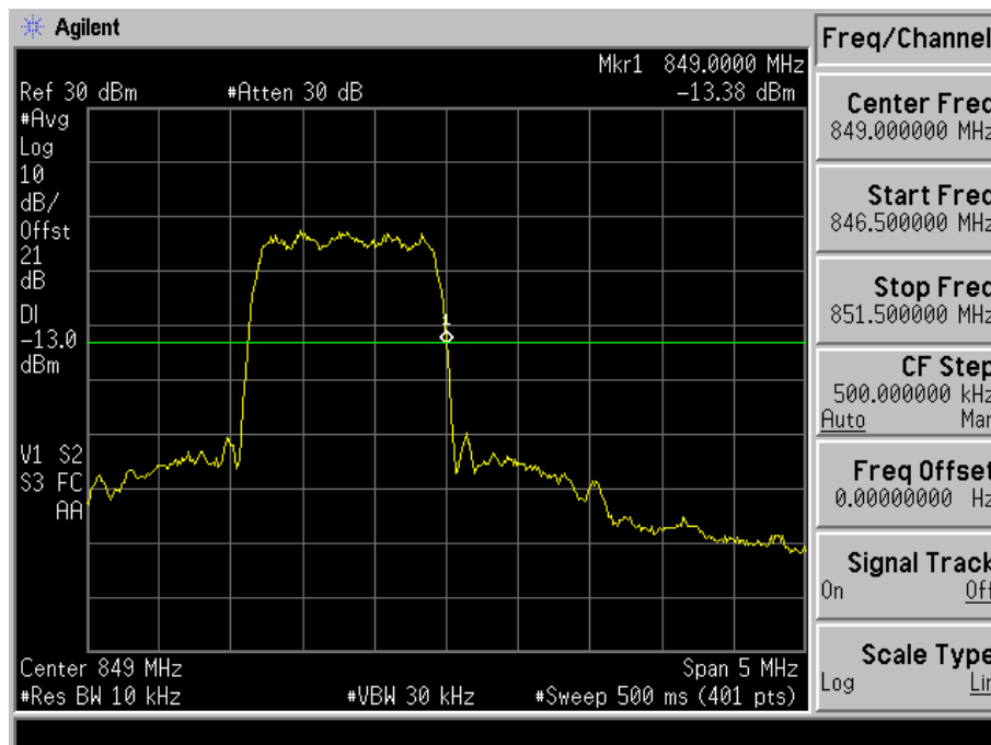
Fig. 4-11 Band edge measurements for mode 1(Ch. 777).
