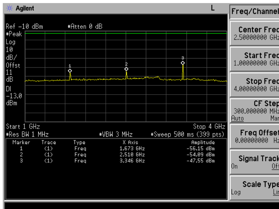
Fig. 5-16(b) Conducted spurious emission for mode 1(Ch. 384).
