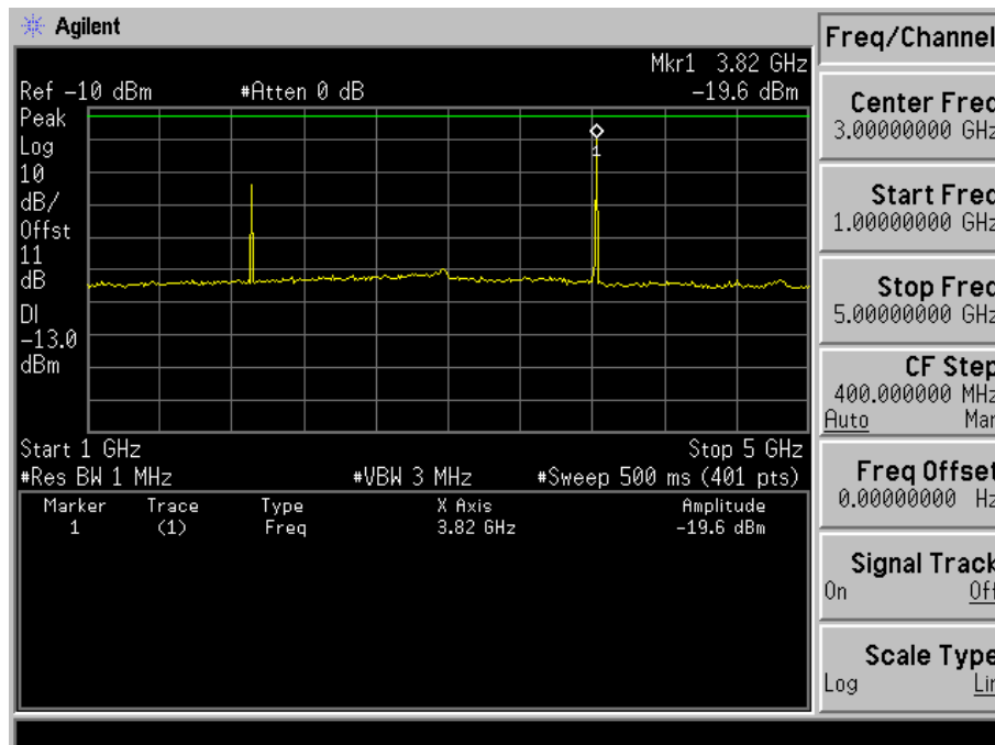
Fig. 5-14(b) Conducted spurious emission for mode 4(Ch. 1175).
