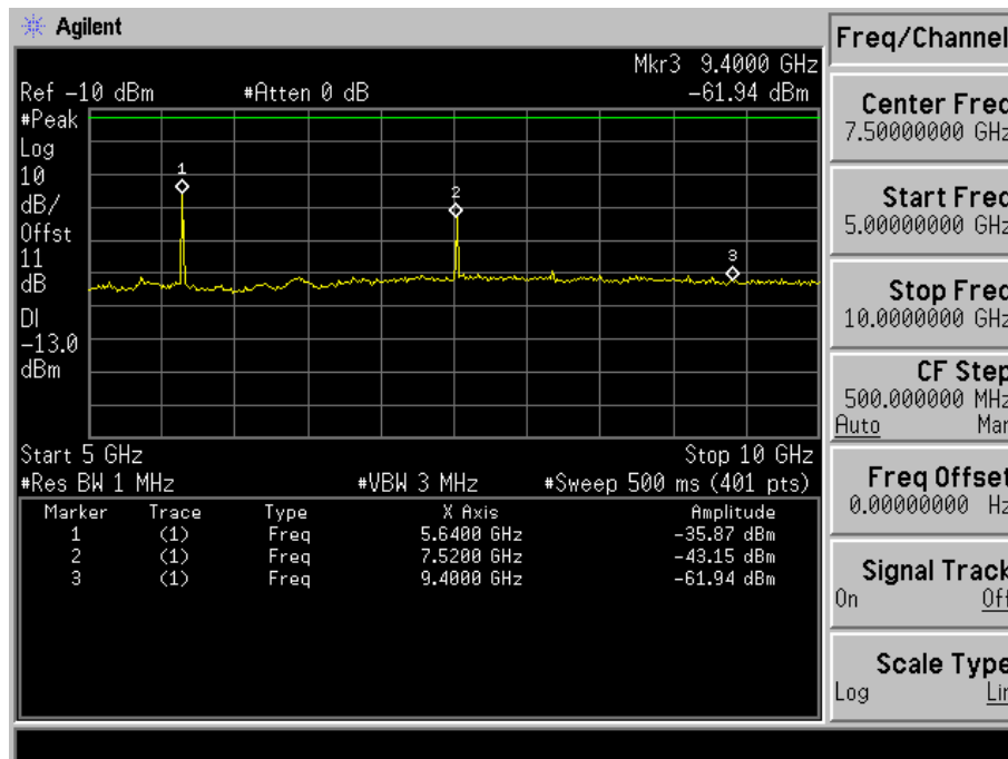
Fig. 5-7(c) Conducted spurious emission for mode 2(Ch. 600).
