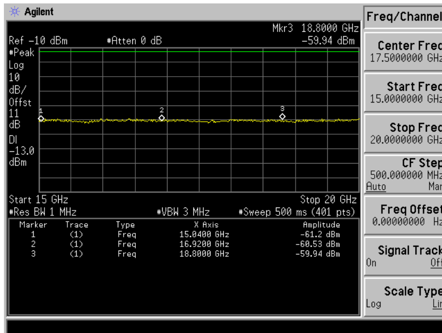
Fig. 5-7(e) Conducted spurious emission for mode 2(Ch. 600).
