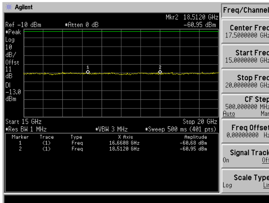
Fig. 5-6(e) Conducted spurious emission for mode 2(Ch. 25).
