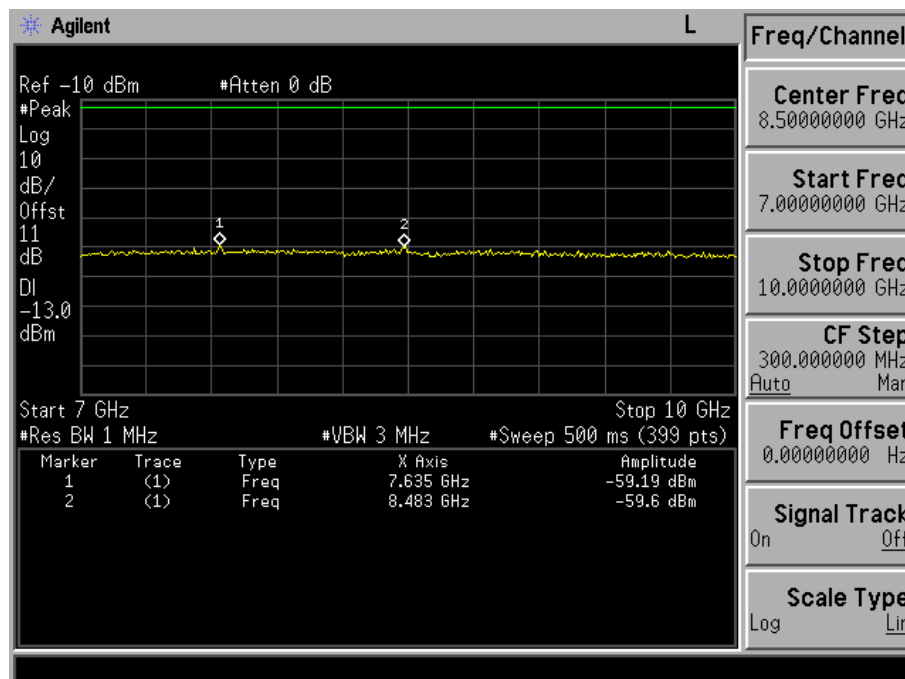
Fig. 5-23(d) Conducted spurious emission for mode 3(Ch. 777).
