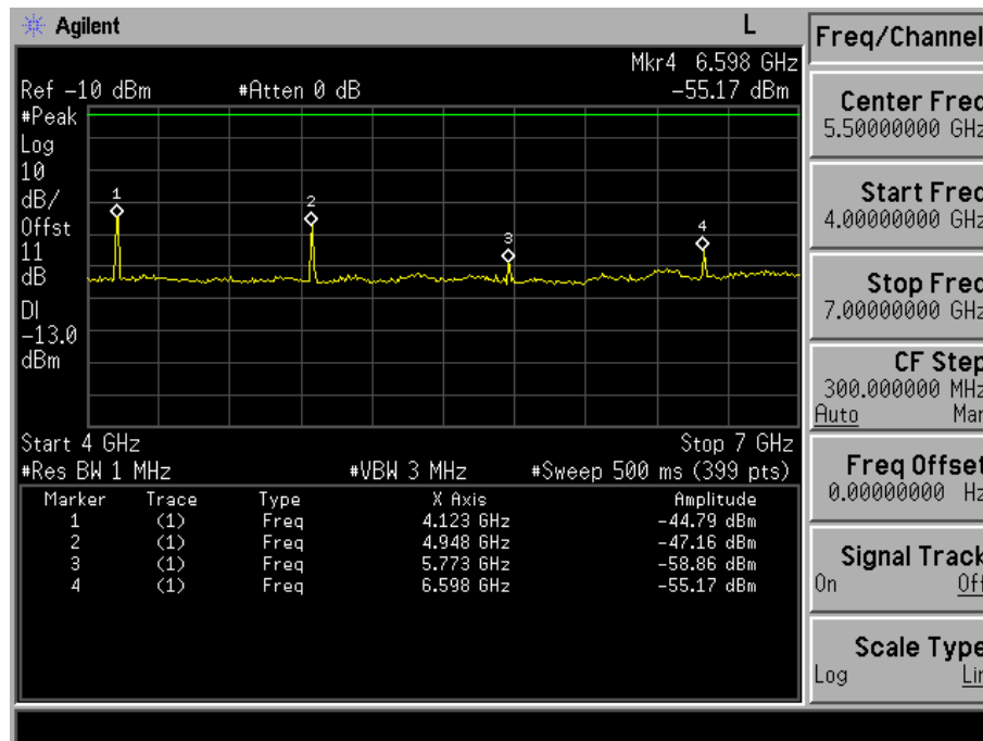
Fig. 5-9(c) Conducted spurious emission for mode 3(Ch. 1013).
