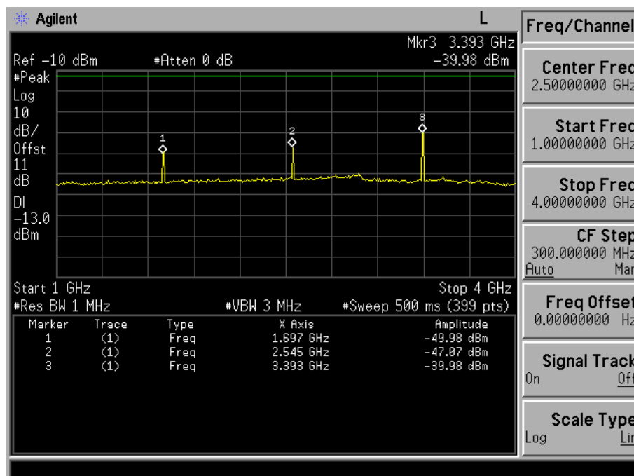
Fig. 5-11(b) Conducted spurious emission for mode 3(Ch. 777).
