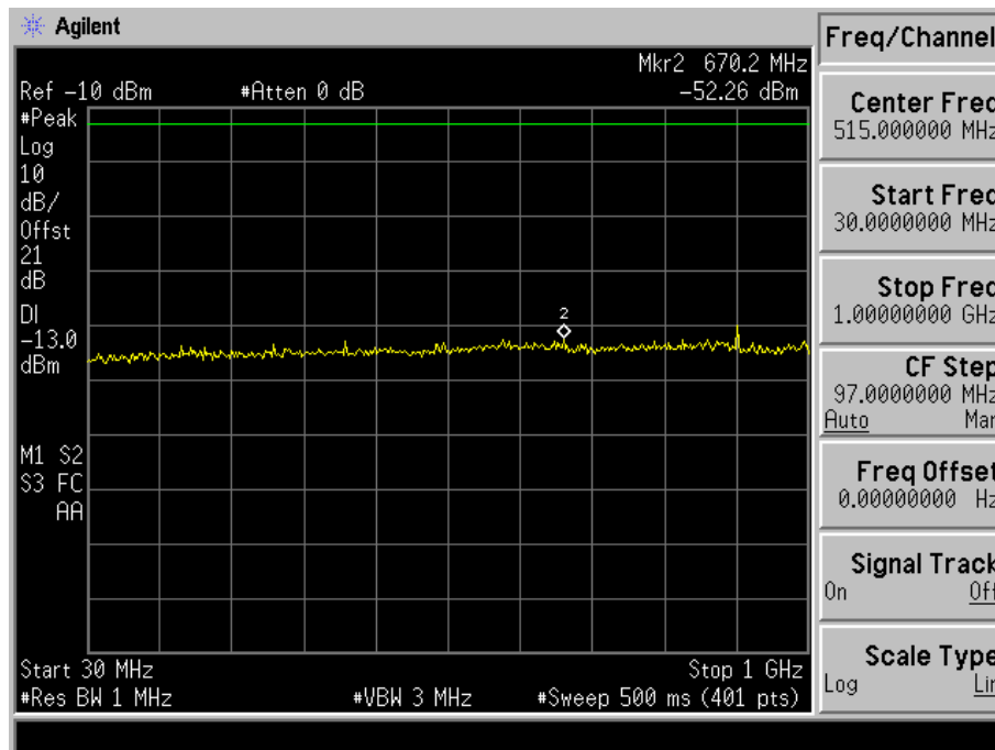
Fig. 5-26(a) Conducted spurious emission for mode 4(Ch. 1175).
