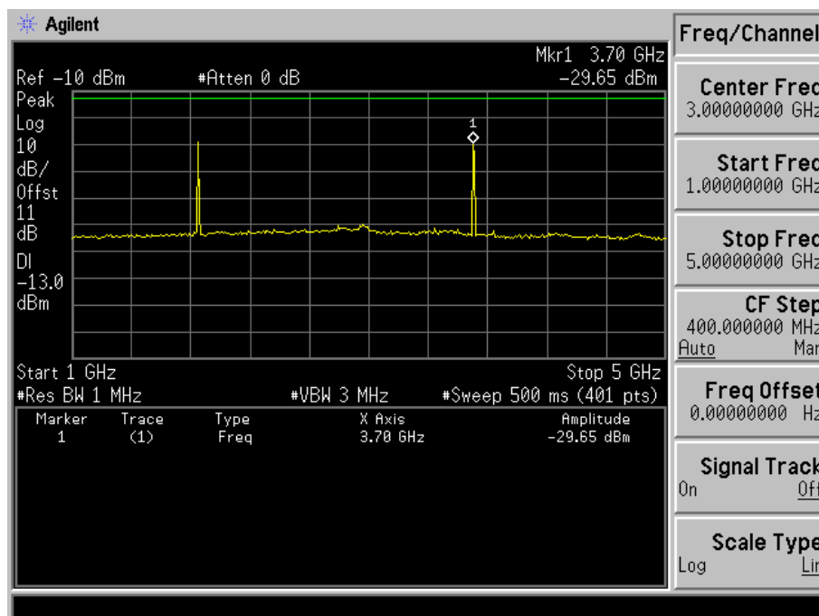
Fig. 5-12(b) Conducted spurious emission for mode 4(Ch. 25).
