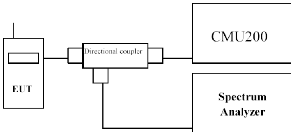
Fig. 4-1 Test setup.
