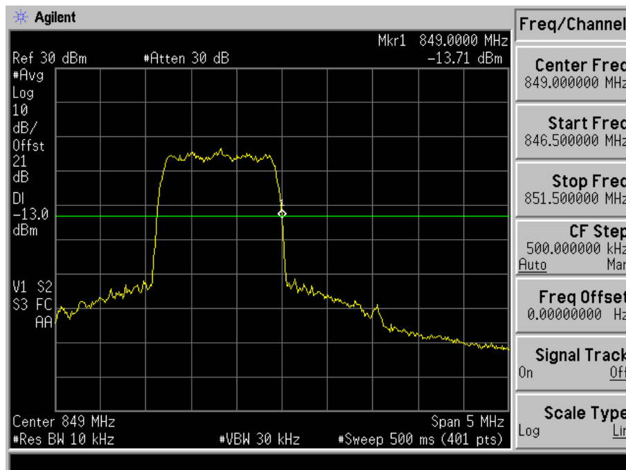
Fig. 4-15 Band edge measurements for mode 3(Ch. 777).
