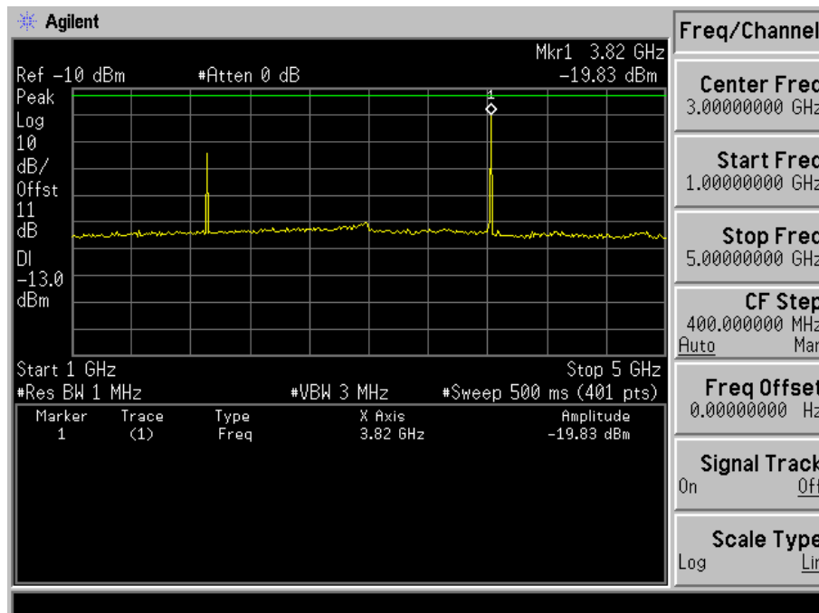
Fig. 5-20(b) Conducted spurious emission for mode 2(Ch. 1175).
