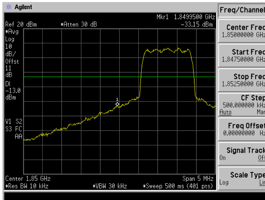
Fig. 4-4 Band edge measurements for mode 2(Ch. 25).
