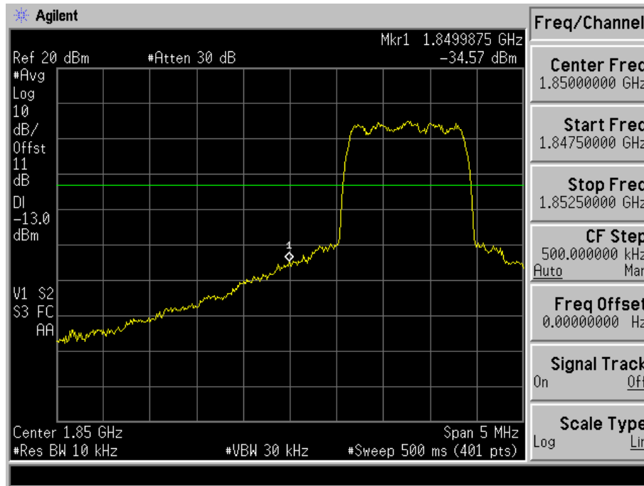
Fig. 4-8 Band edge measurements for mode 4(Ch. 25).
