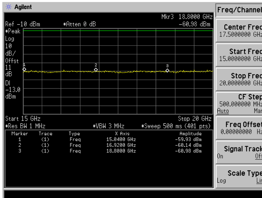
Fig. 5-25(e) Conducted spurious emission for mode 4(Ch. 600).
