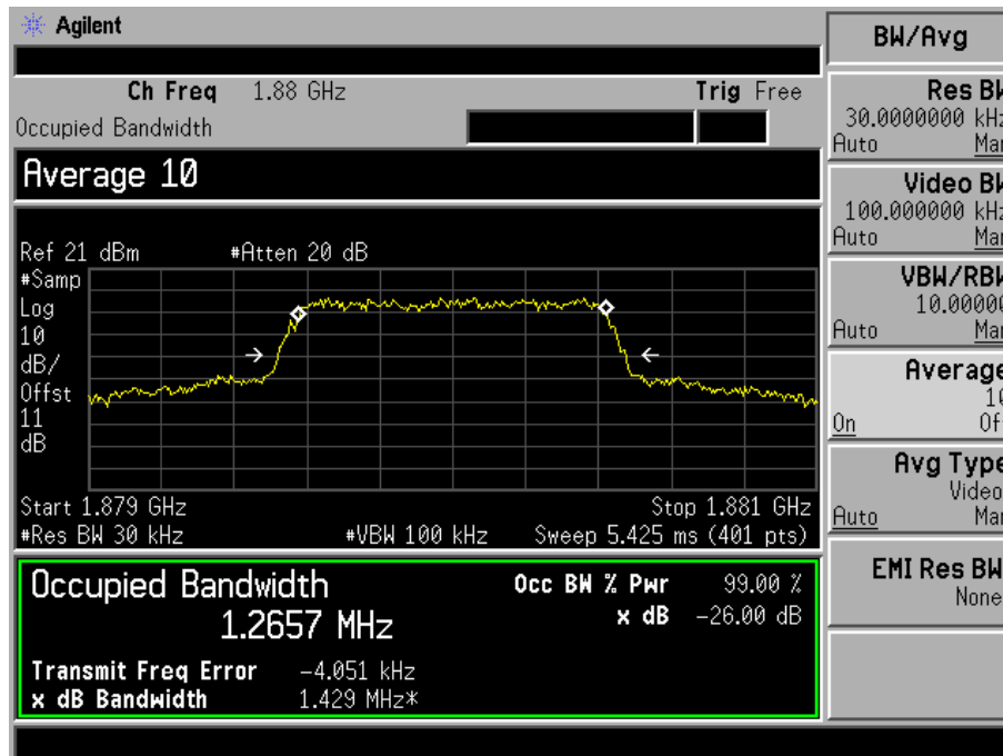
Fig. 3-6 Occupied Bandwidth for mode 2(Ch. 600).
