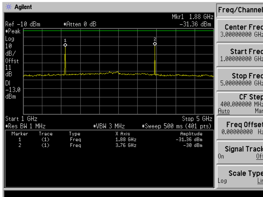
Fig. 5-7(b) Conducted spurious emission for mode 2(Ch. 600).
