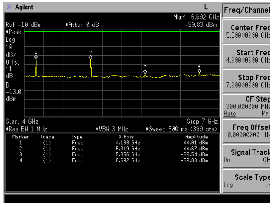
Fig. 5-10(c) Conducted spurious emission for mode 3(Ch. 384).
