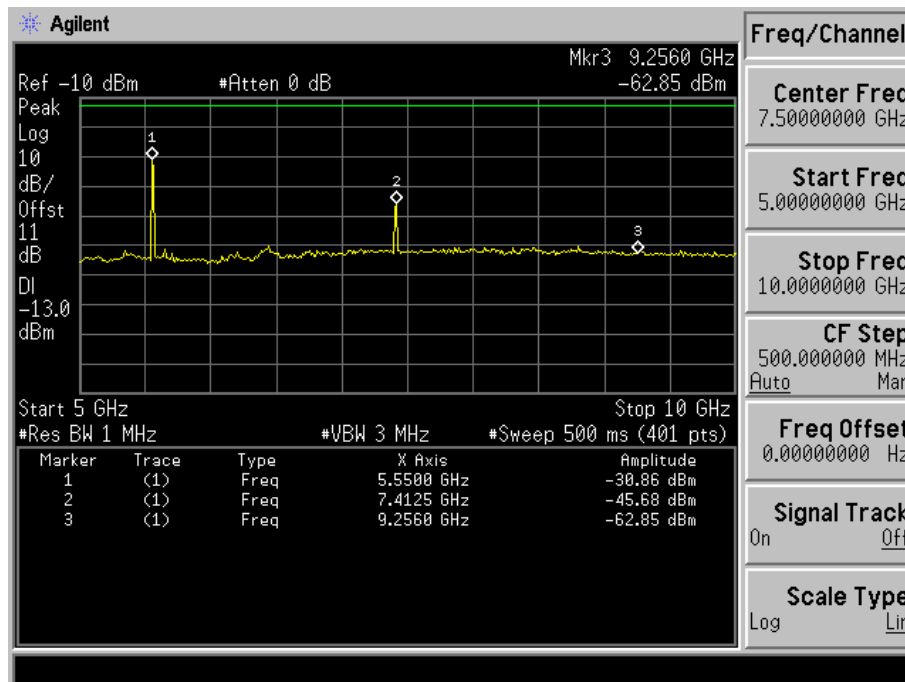
Fig. 5-18(c) Conducted spurious emission for mode 2(Ch. 25).
