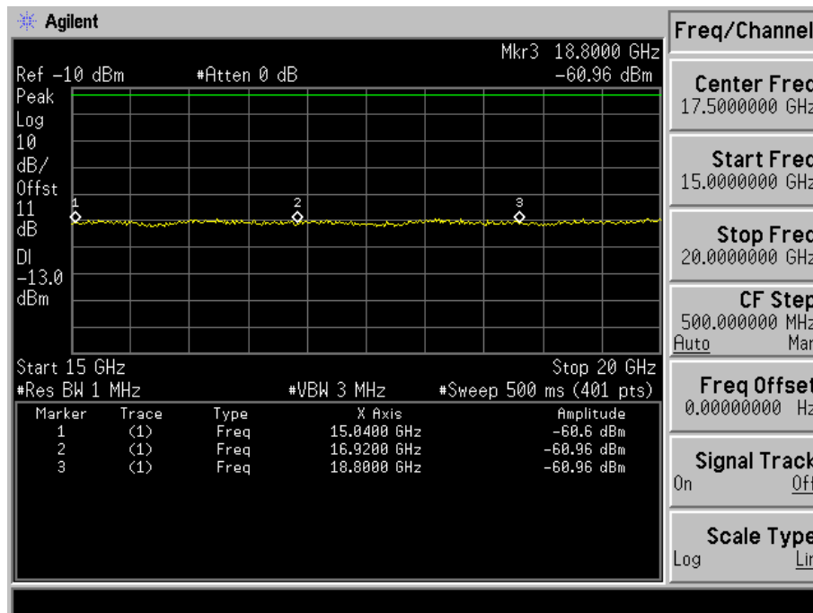
Fig. 5-19(e) Conducted spurious emission for mode 2(Ch. 600).
