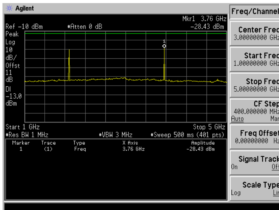
Fig. 5-13(b) Conducted spurious emission for mode 4(Ch. 600).
