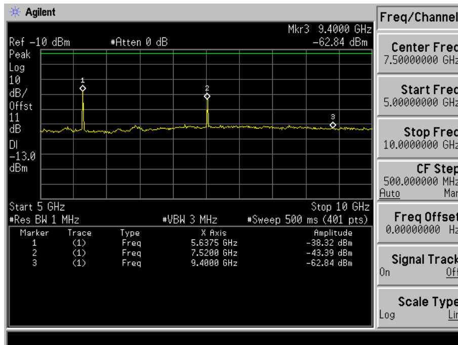
Fig. 5-19(c) Conducted spurious emission for mode 2(Ch. 600).
