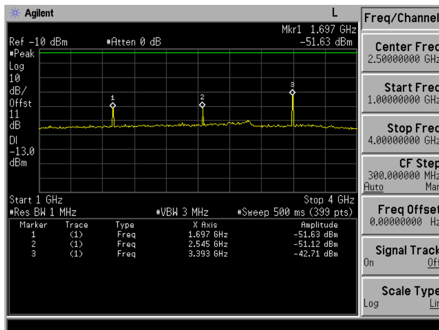
Fig. 5-17(b) Conducted spurious emission for mode 1(Ch. 777).
