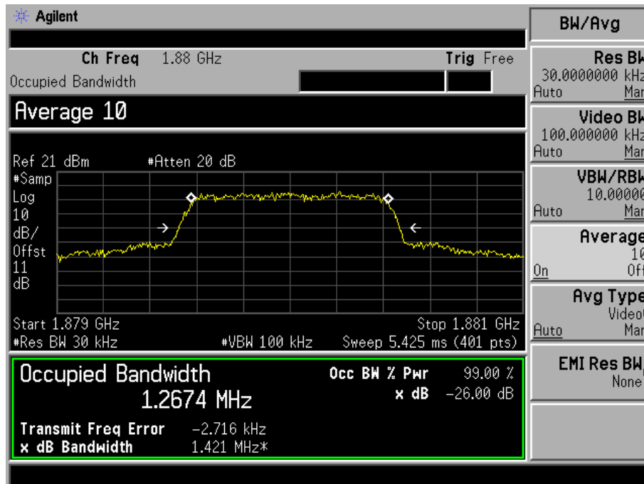
Fig. 3-12 Occupied Bandwidth for mode 4(Ch. 600).
