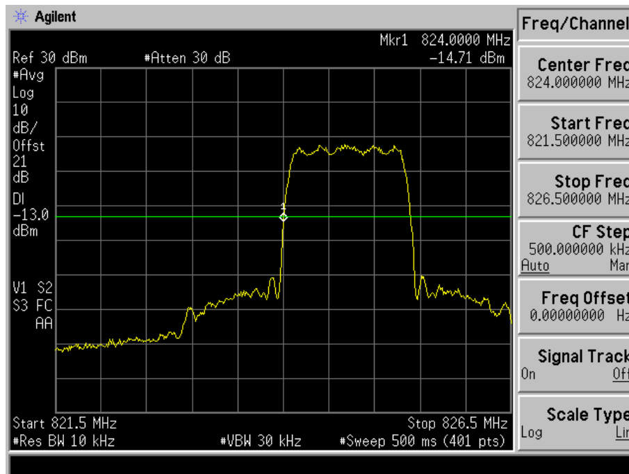
Fig. 4-10 Band edge measurements for mode 1(Ch. 1013).
