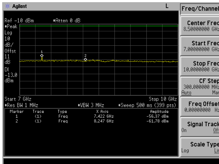
Fig. 5-15(d) Conducted spurious emission for mode 1(Ch. 1013).
