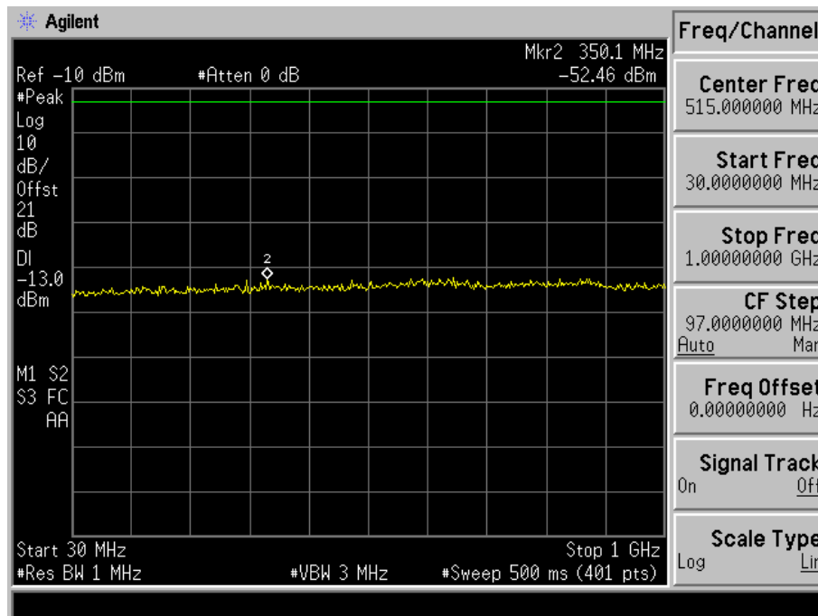
Fig. 5-18(a) Conducted spurious emission for mode 2(Ch. 25).
