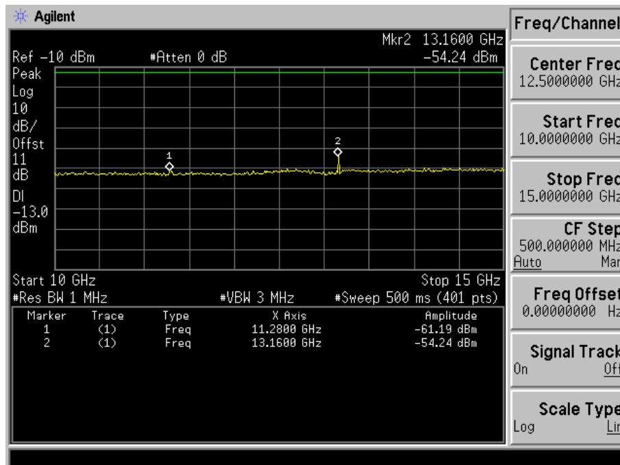
Fig. 5-13(d) Conducted spurious emission for mode 4(Ch. 600).
