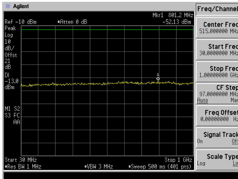
Fig. 5-6(a) Conducted spurious emission for mode 2(Ch. 25).
