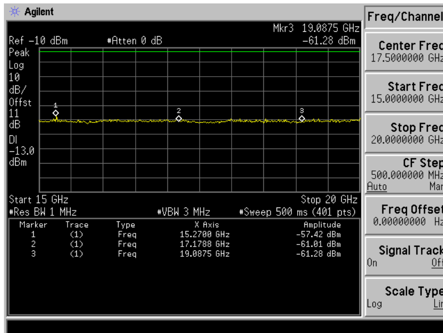
Fig. 5-20(e) Conducted spurious emission for mode 2(Ch. 1175).
