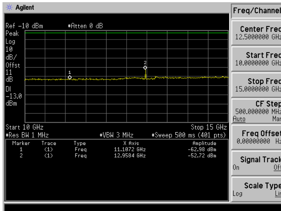
Fig. 5-12(d) Conducted spurious emission for mode 4(Ch. 25).
