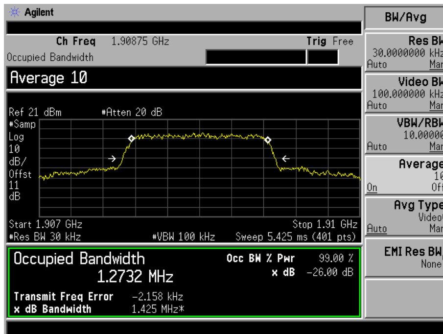
Fig. 3-13 Occupied Bandwidth for mode 4(Ch. 1175).
