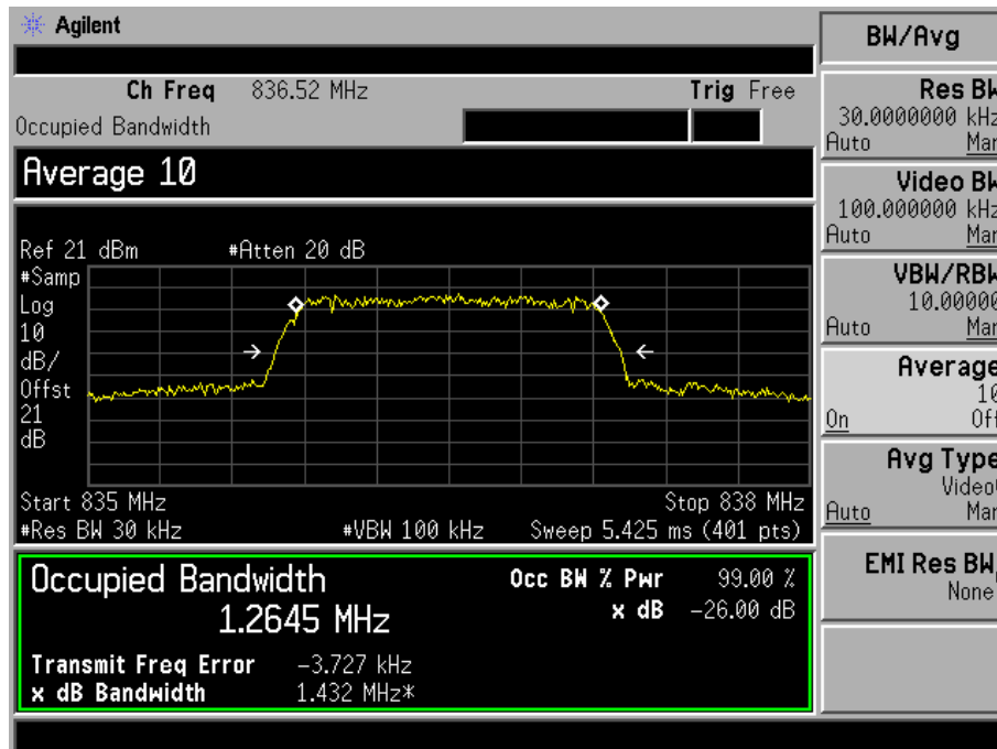
Fig. 3-9 Occupied Bandwidth for mode 3(Ch. 384).
