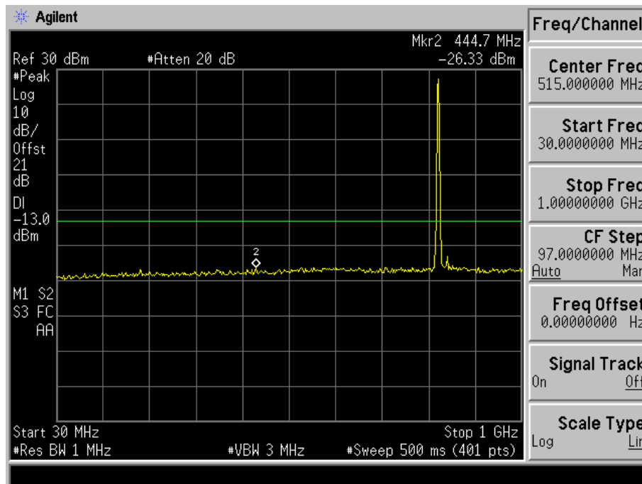
Fig. 5-17(a) Conducted spurious emission for mode 1(Ch. 777).
