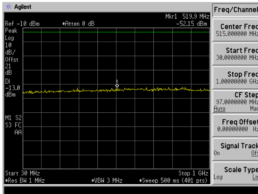
Fig. 5-14(a) Conducted spurious emission for mode 4(Ch. 1175).
