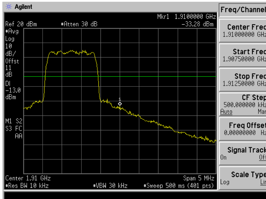
Fig. 4-17 Band edge measurements for mode 4(Ch. 1175).
