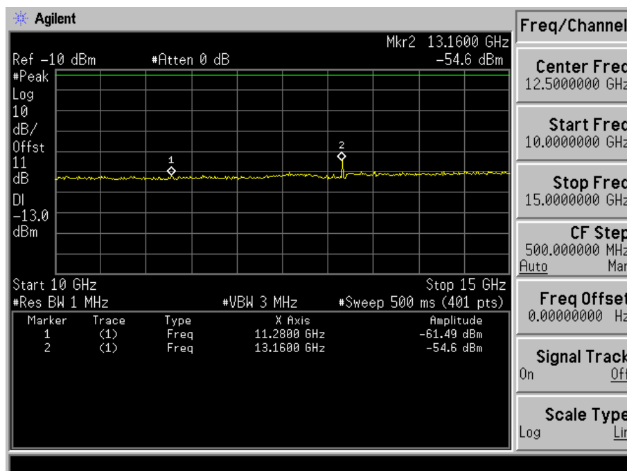
Fig. 5-25(d) Conducted spurious emission for mode 4(Ch. 600).
