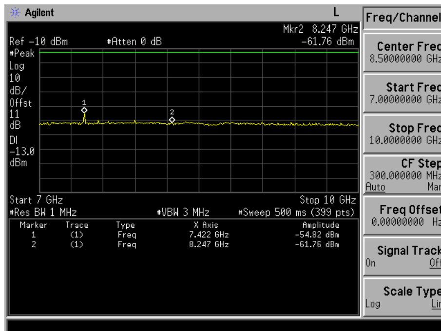
Fig. 5-9(d) Conducted spurious emission for mode 3(Ch. 1013).
