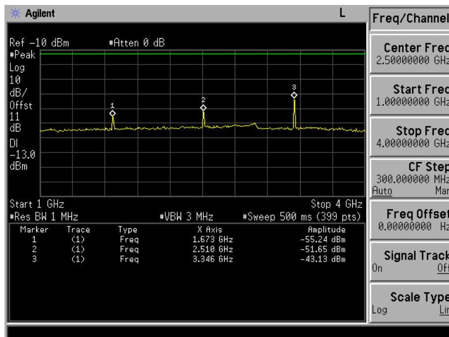
Fig. 5-10(b) Conducted spurious emission for mode 3(Ch. 384).
