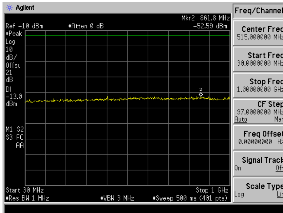
Fig. 5-24(a) Conducted spurious emission for mode 4(Ch. 25).
