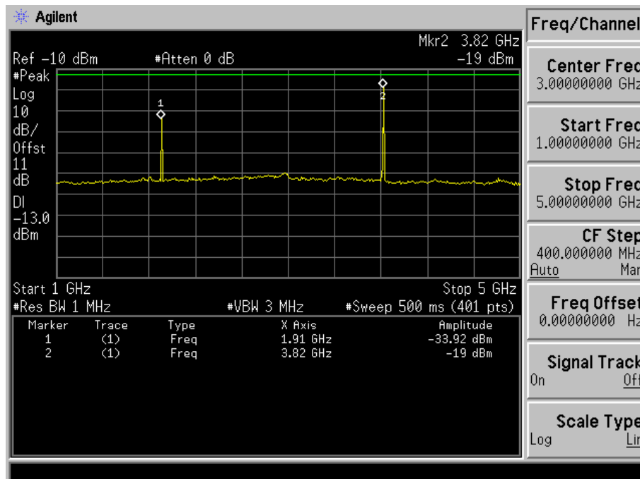
Fig. 5-26(b) Conducted spurious emission for mode 4(Ch. 1175).
