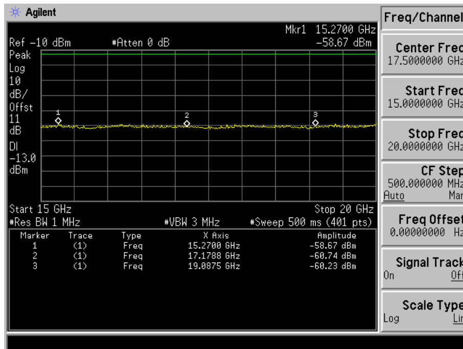
Fig. 5-14(e) Conducted spurious emission for mode 4(Ch. 1175).
