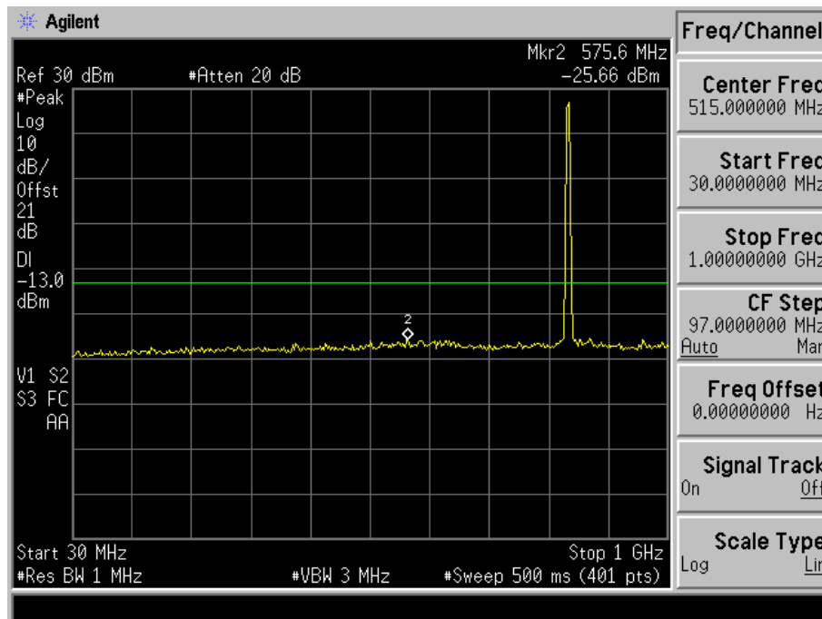
Fig. 5-15(a) Conducted spurious emission for mode 1(Ch. 1013).
