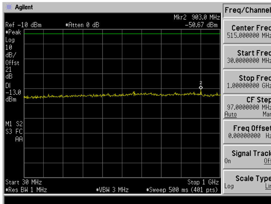
Fig. 5-20(a) Conducted spurious emission for mode 2(Ch. 1175).
