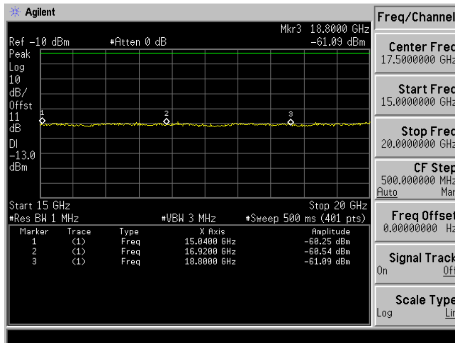
Fig. 5-13(e) Conducted spurious emission for mode 4(Ch. 600).
