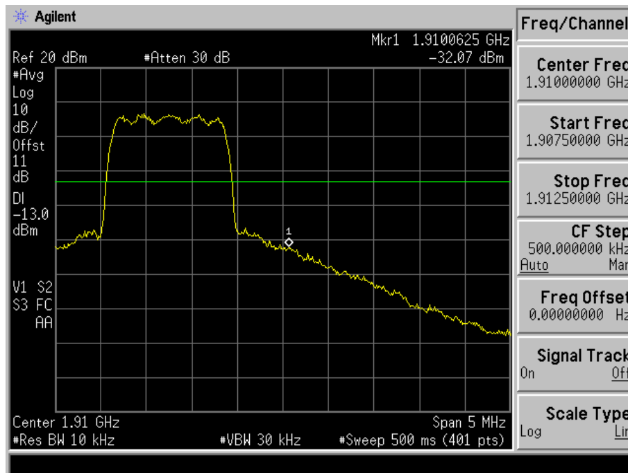
Fig. 4-5 Band edge measurements for mode 2(Ch. 1175).
