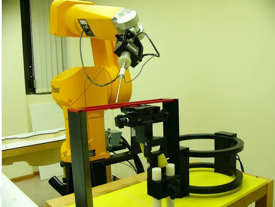
Fig.1 Photograph of the HAC measurement System
