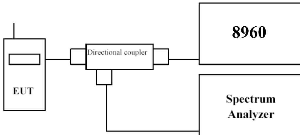
Fig. 3-1 Test setup.
