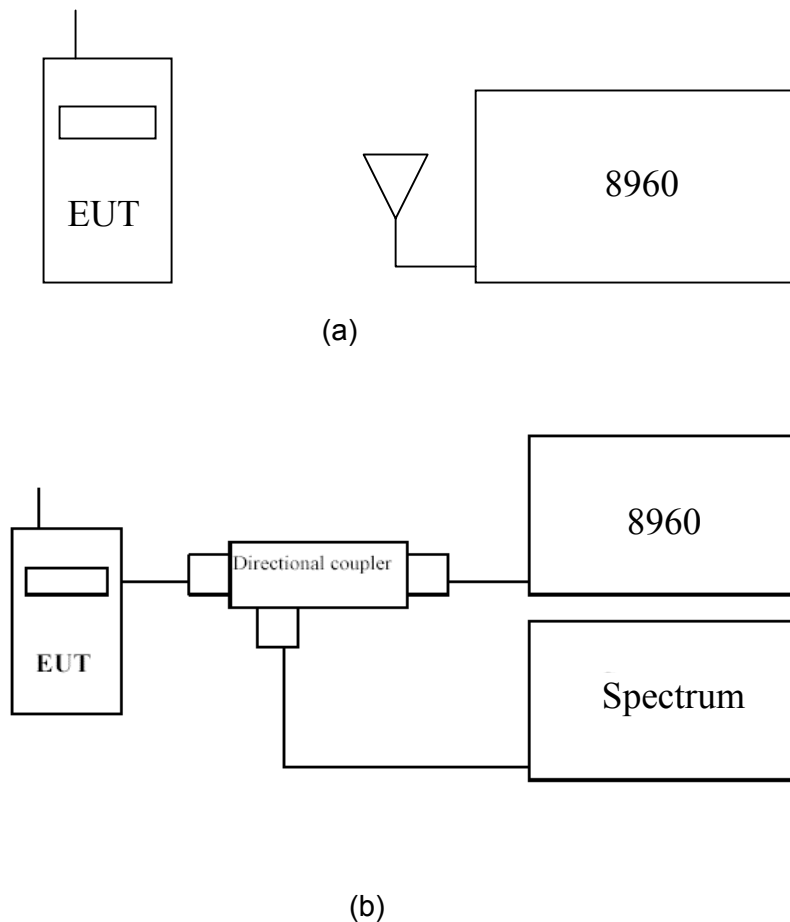
Fig. 1-1 Configuration of (a) Radiated (b) Conducted Emission measurement.
