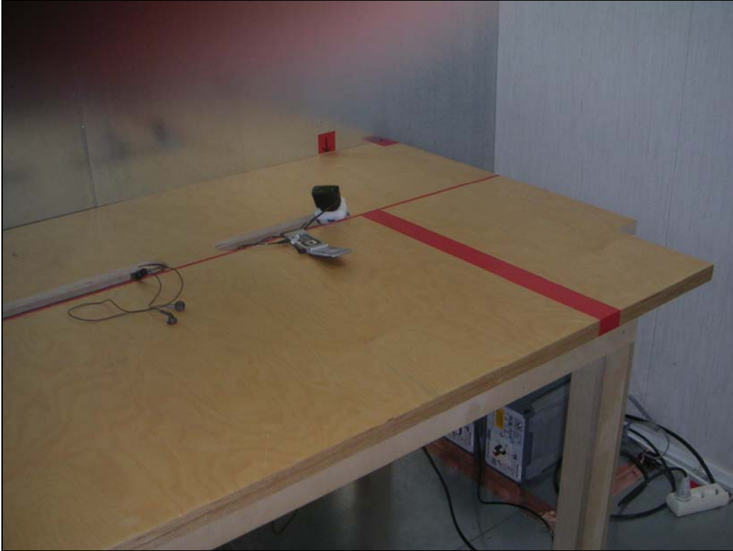
Picture 3 AC powerline conducted emission measurement GSM RX/BT TX
