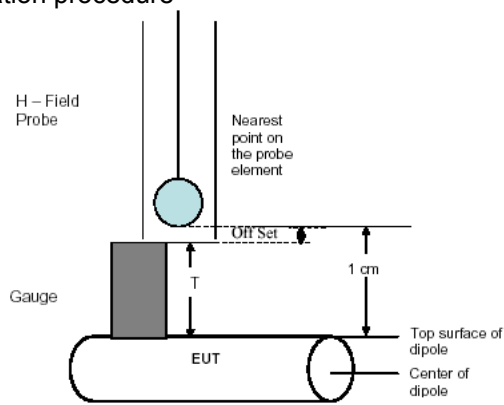
Figure 5. WD dipole calibration procedure
