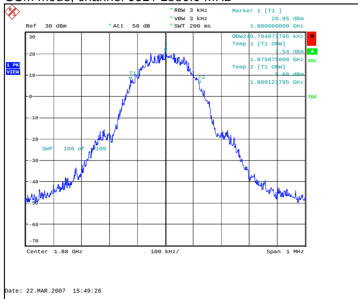
GSM mode, channel 661 / 1880.0 MHz
