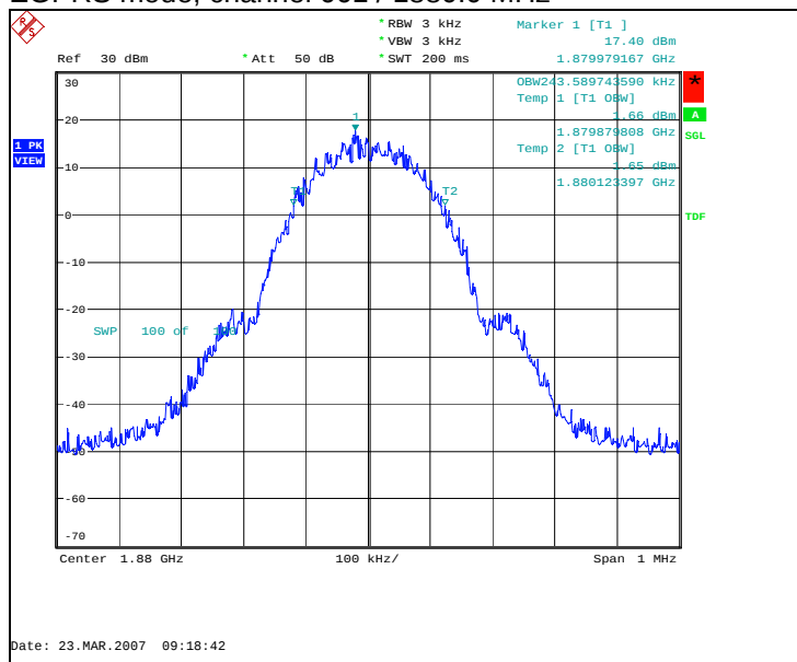
EGPRS mode, channel 661 / 1880.0 MHz
