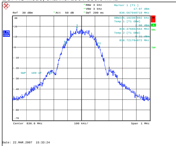
EGPRS mode, channel 190 / 836.6 MHz
