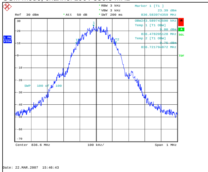
GSM mode, channel 190 / 836.6 MHz
