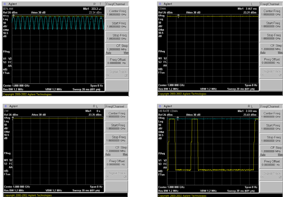
Figure 26 Zero-Span Plots
