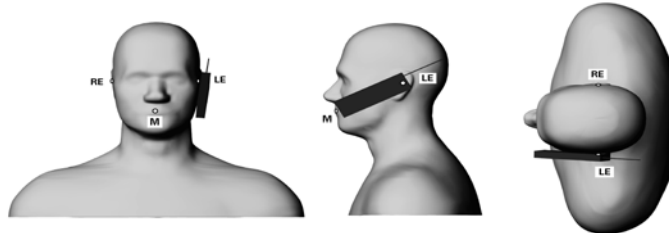
Fig. 5.1.1. Cheek/Touch position
