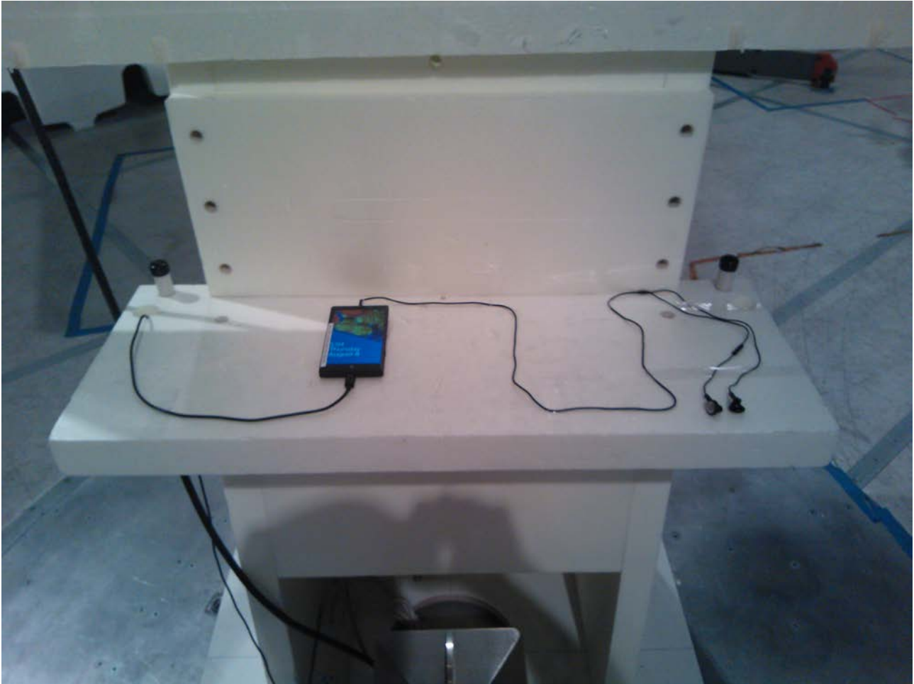
Picture 3. FCC Part 15B Radiated emissions
