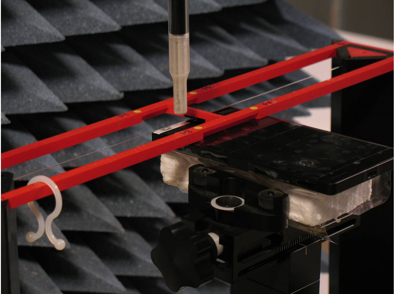
Figure 3: Test Setup Photograph – Near Field Emissions Test
