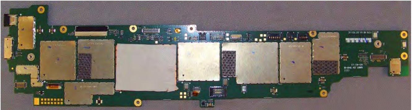
[Main Board w/ Shields]
