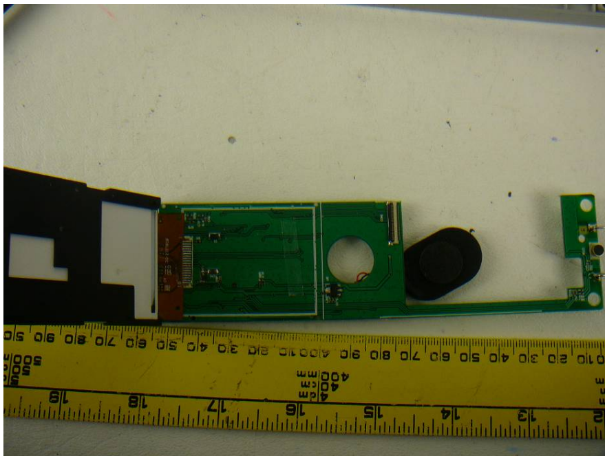
EUT (Handset) – Main Board Top without LCD View
