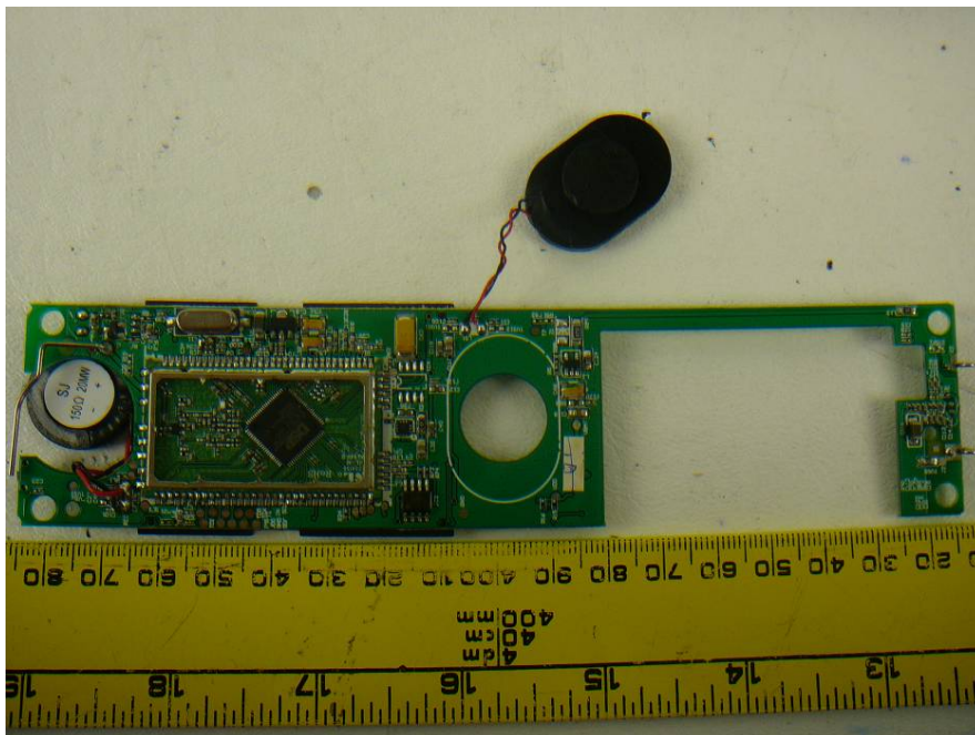
EUT (Handset) – Main Board Bottom Shielding off View
