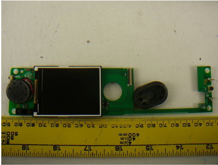
EUT (Handset) – Main Board Top with LCD View
