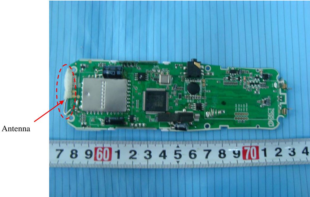
EUT – Main Board with Shielding View
