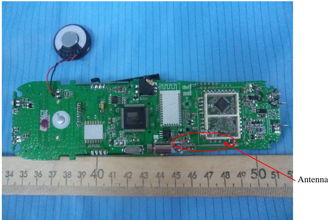
EUT – Handset Main Board Bottom Shielding off View
