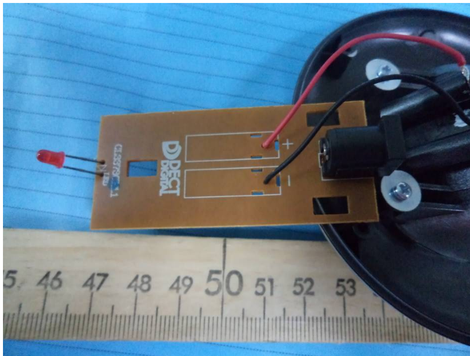
EUT – Charger Main Board Top View
