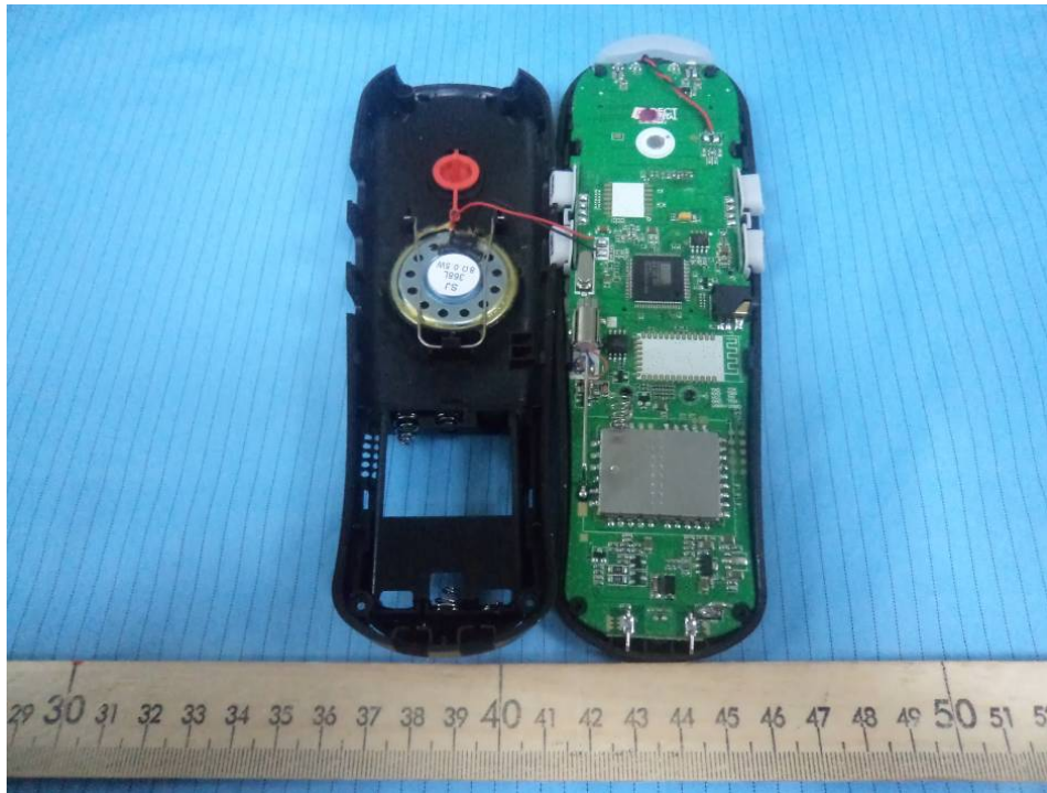
EUT – Handset Main Board Top View
