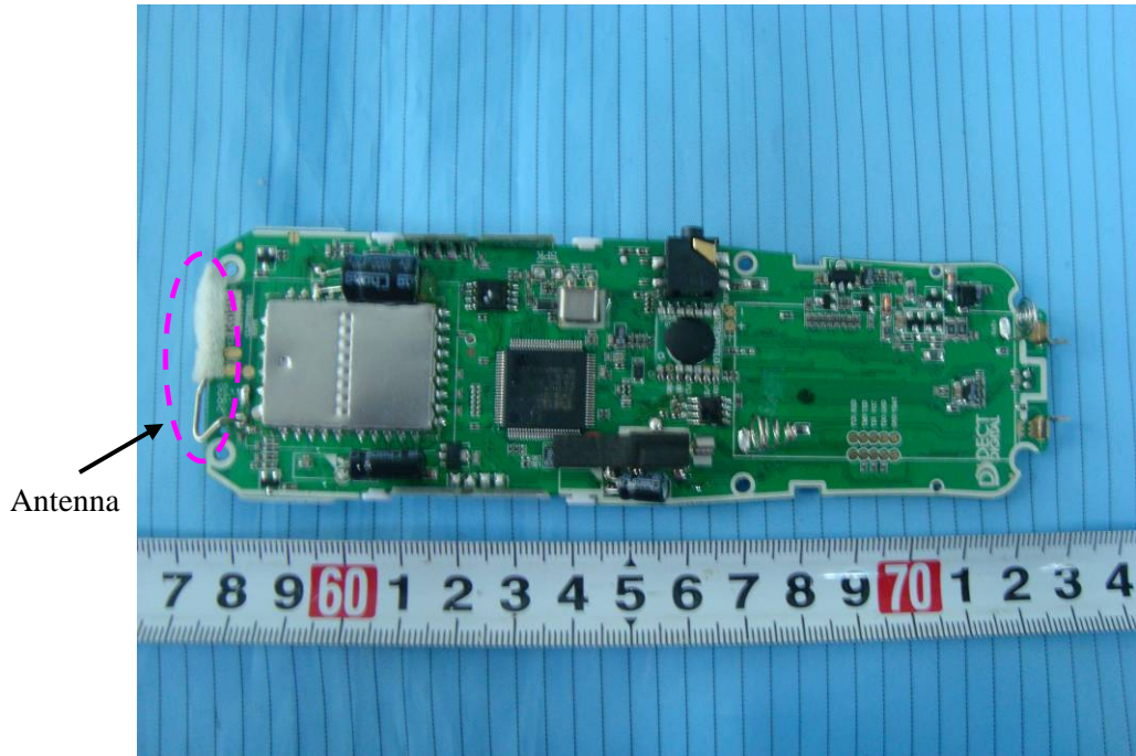
EUT – Main Board with Shielded Cover Top View
