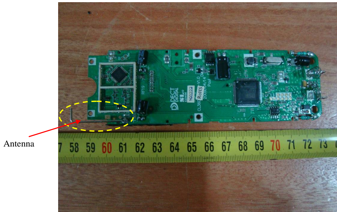
EUT – Main Board Shielding Off Bottom View
