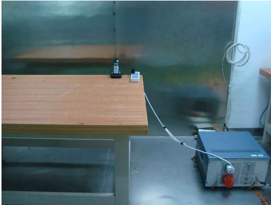
Charging: Conducted Emissions – Side View
