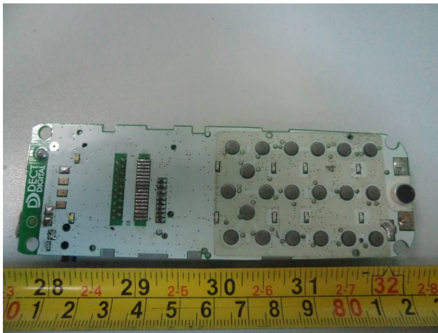
EUT – Main Board without LCD Bottom View
