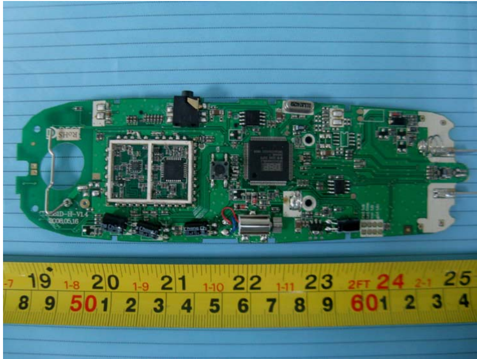
EUT- Main Board Components Bottom View (without shielded cover)
