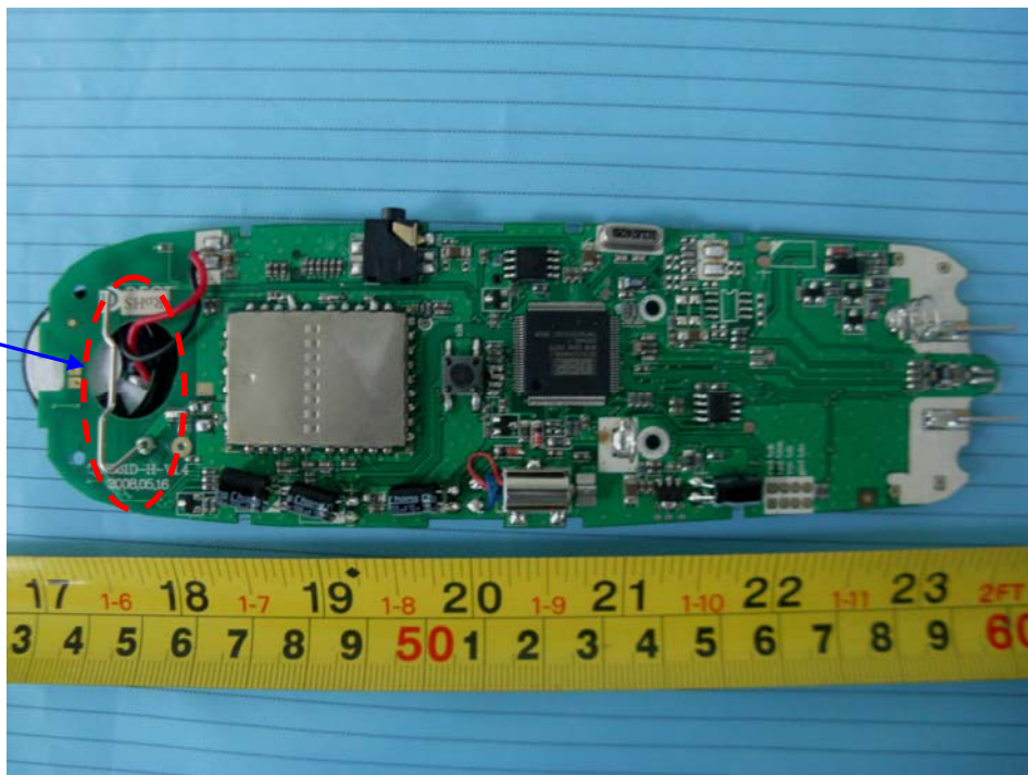
EUT- Main Board Components Bottom View (with shielded cover)
