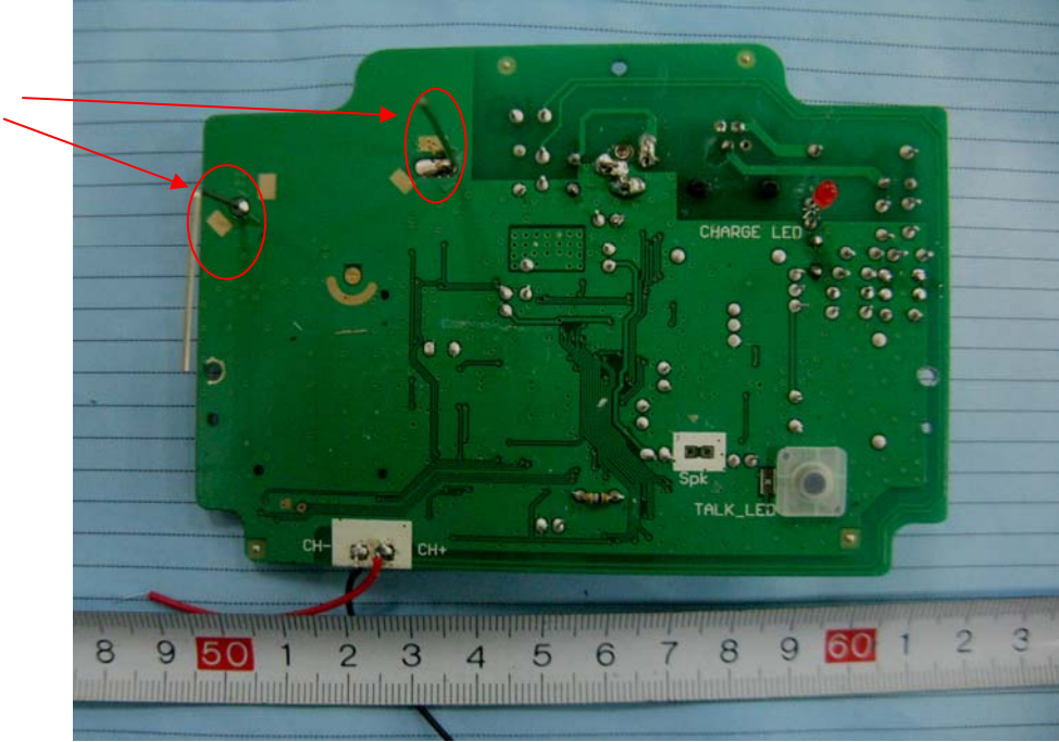
EUT – Main Board Bottom Components View
