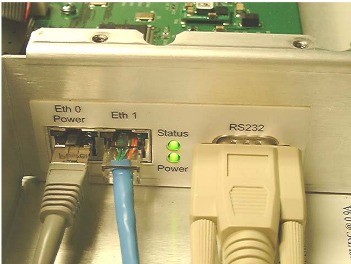
Figure 4 IO Ports
