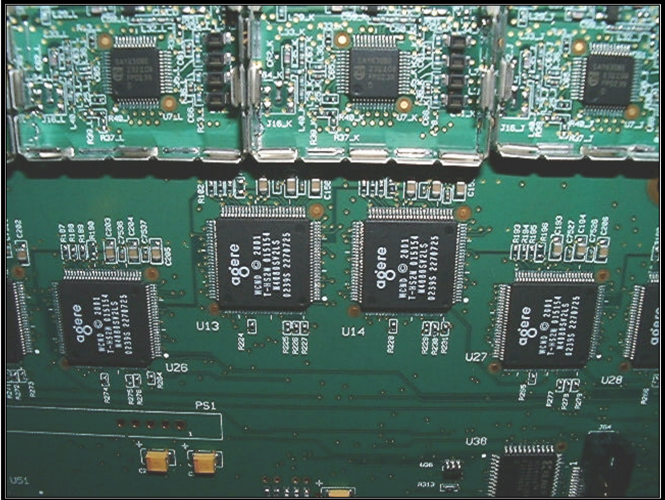
PHOTOGRAPH 58: BASEBAND CHIPS
