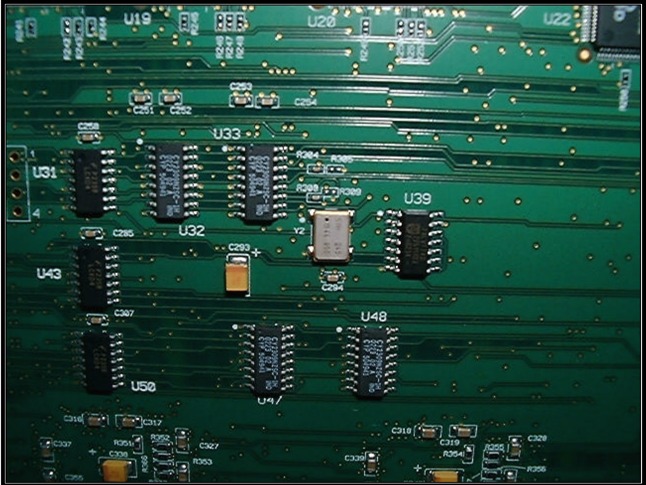
PHOTOGRAPH 59: CRYSTAL OSCILLATOR
