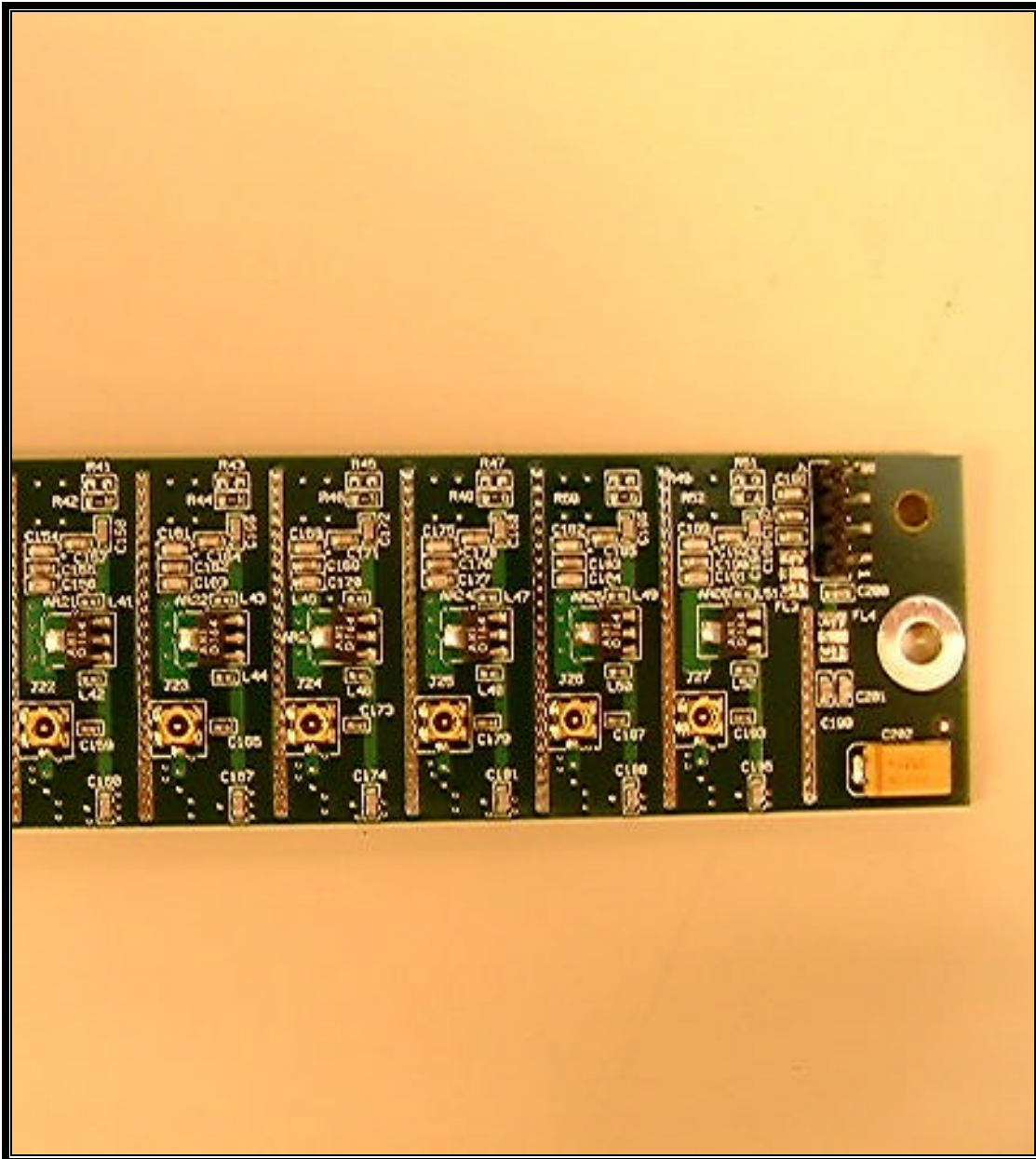
PHOTOGRAPH 40: SOSA BOARD-SIDE 1 RIGHT HALF
