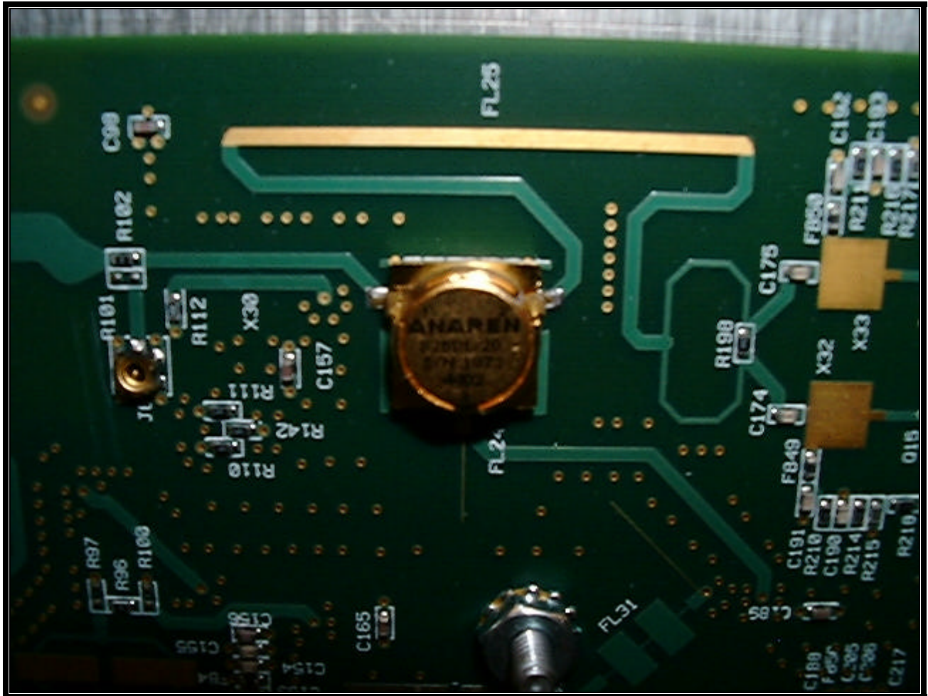
PHOTOGRAPH 37: ANTENNA BOARD CIRCULATOR
