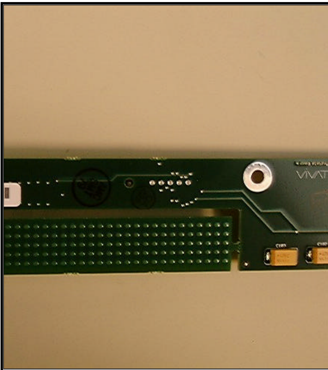
PHOTOGRAPH 39: SOSA BOARD-SIDE 1 LEFT HALF
