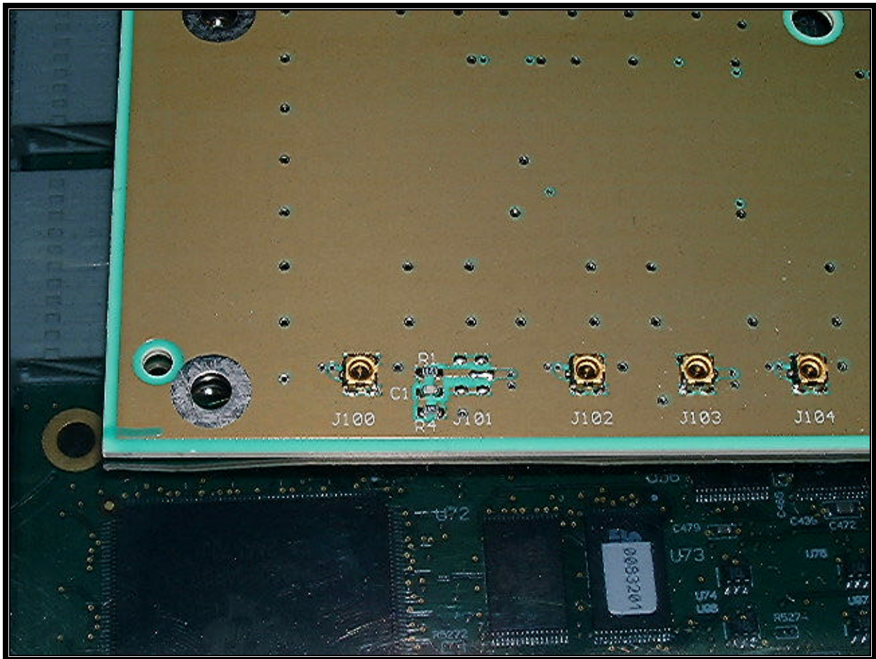
PHOTOGRAPH 21: ALFRED BOARD CONNECTORS
