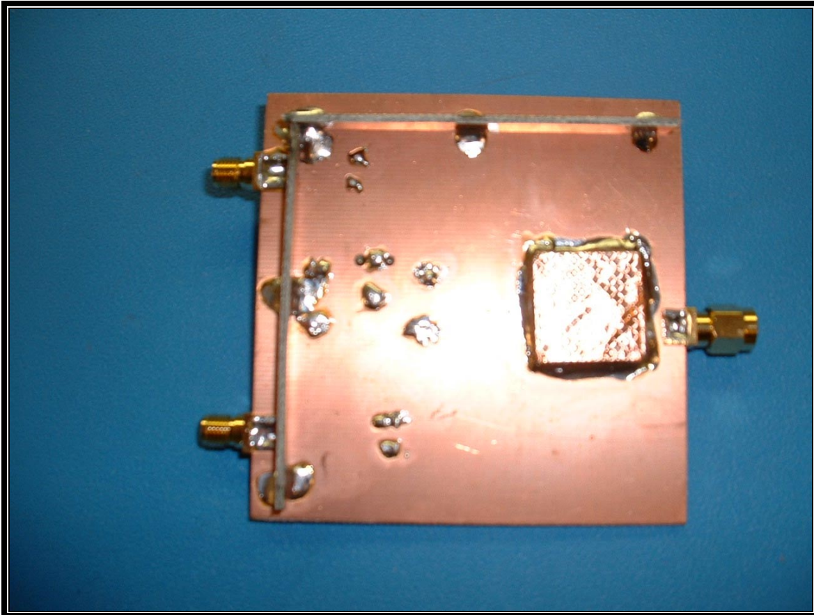
PHOTOGRAPH 47: RFIO BOTTOM
