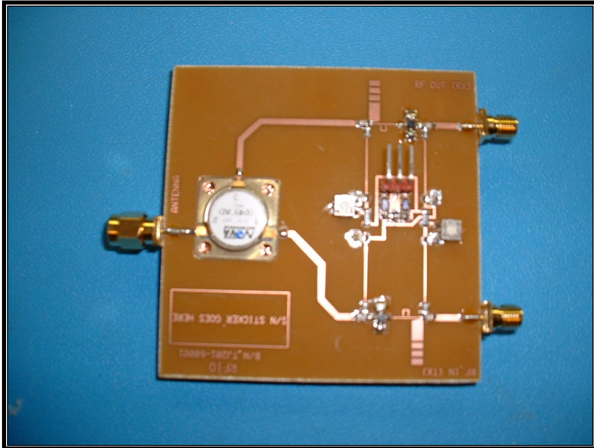
PHOTOGRAPH 46: RFIO TOP
