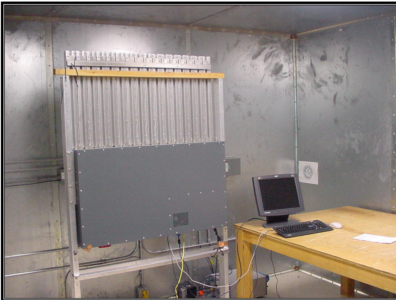
PHOTOGRAPH 6: CONDUCTED EMISSION REAR VIEW WORST-CASE CONFIGURATION
