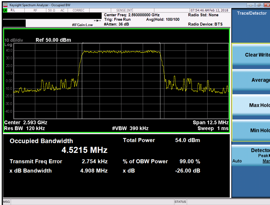
Plot 7-114. Occupied Bandwidth Plot (Band 41 - 5.0MHz 16-QAM)
