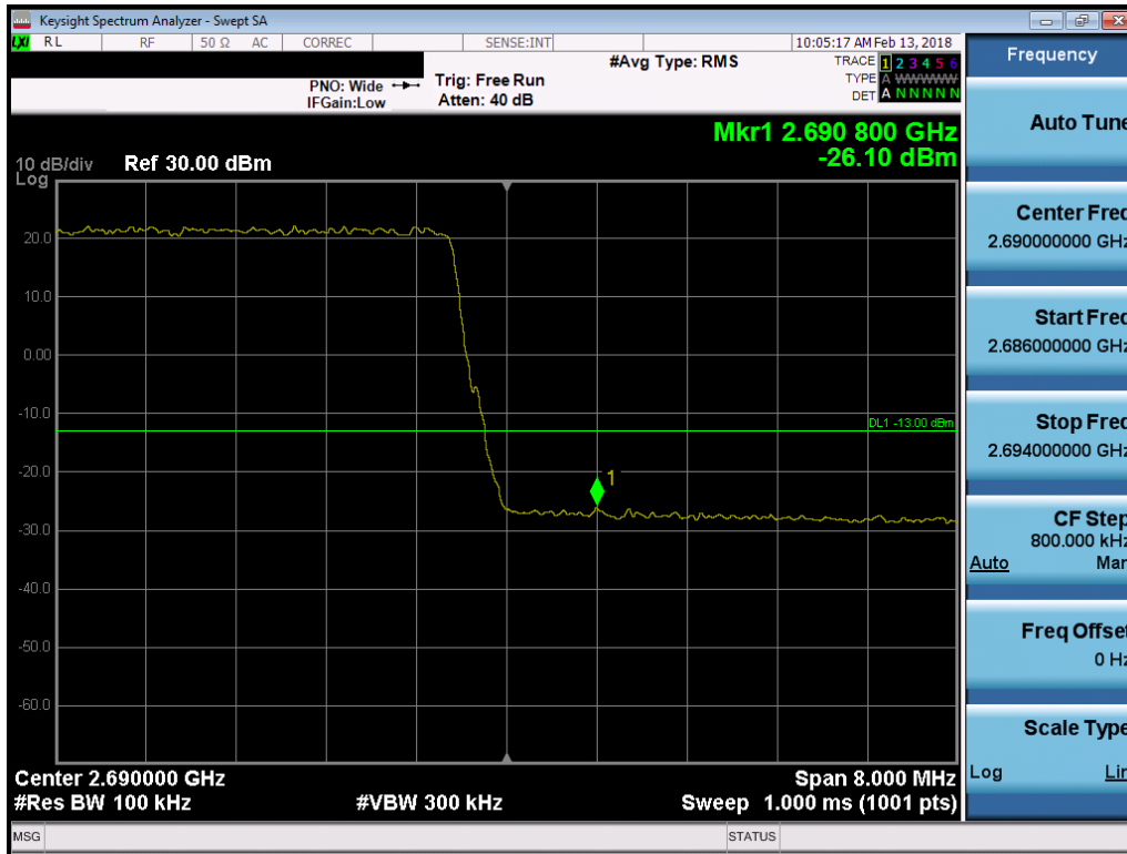
Plot 7-177. Upper Band Edge Plot (Band 41 - 10.0MHz 256-QAM)
