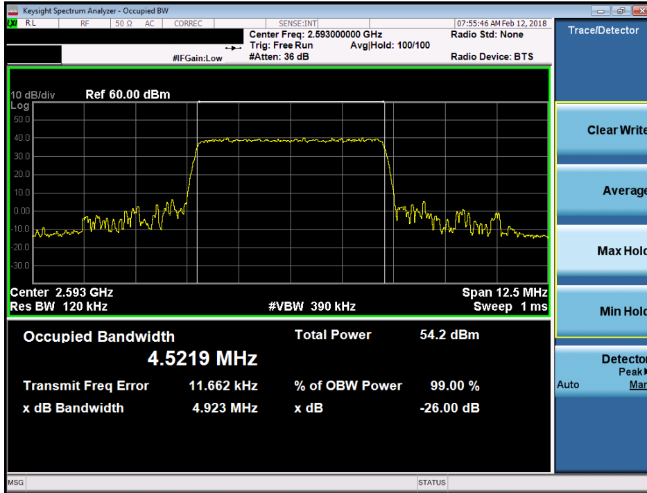
Plot 7-113. Occupied Bandwidth Plot (Band 41 - 5.0MHz QPSK)
