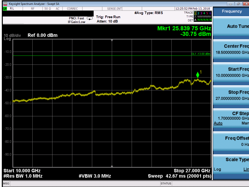
Plot 7-131. Conducted Spurious Plot (Band 41 - 5.0MHz QPSK – Low Channel)
