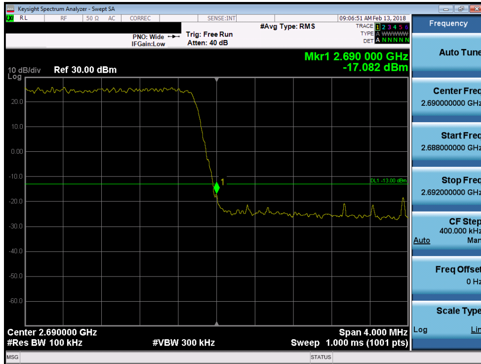
Plot 7-149. Upper Band Edge Plot (Band 41 - 5.0MHz QPSK)
