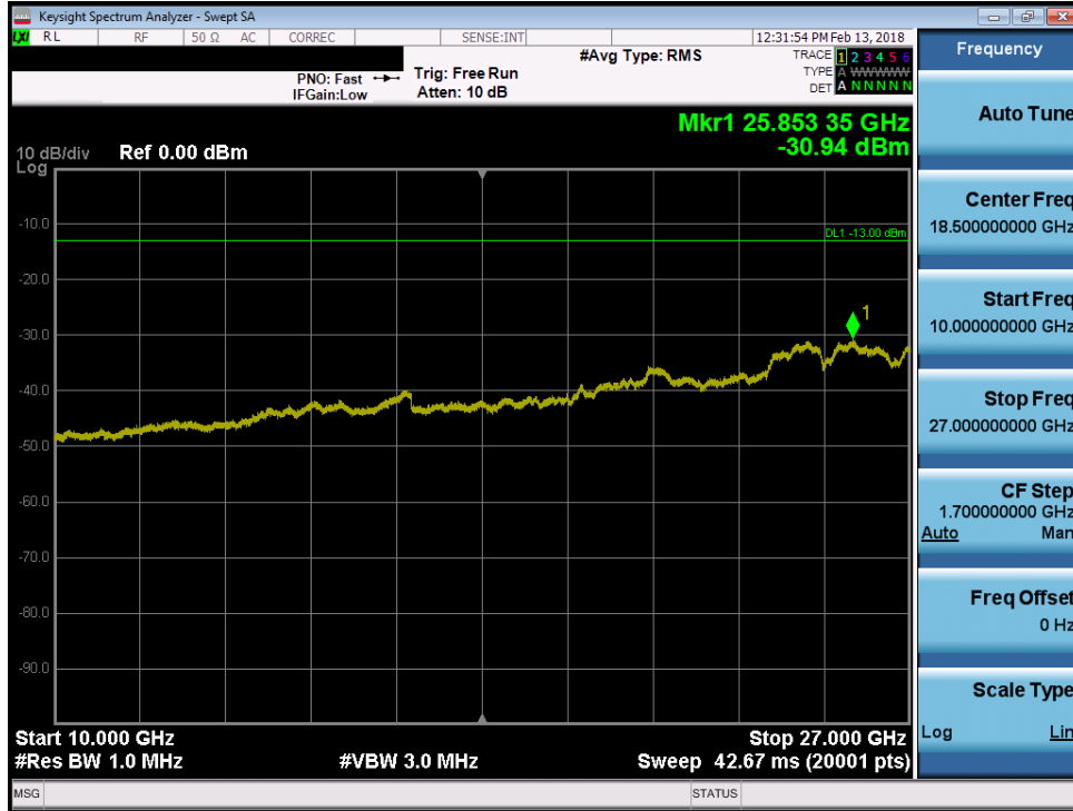
Plot 7-137. Conducted Spurious Plot (Band 41 - 5.0MHz QPSK – High Channel)
