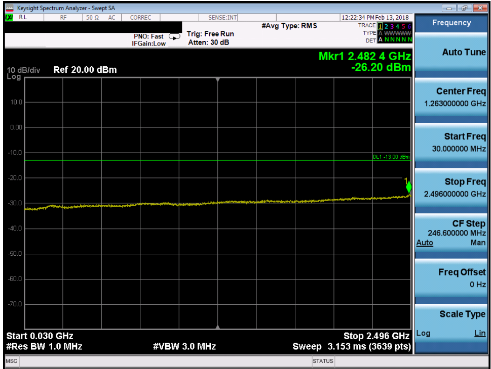
Plot 7-129. Conducted Spurious Plot (Band 41 - 5.0MHz QPSK – Low Channel)
