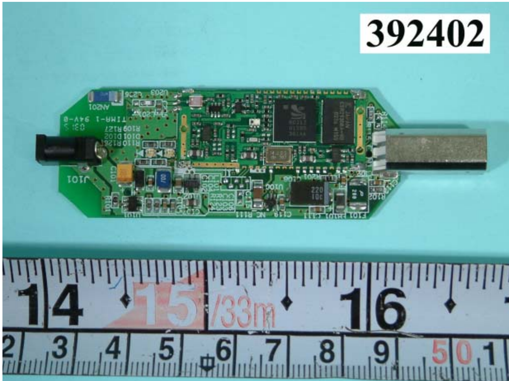
FRONT SIDE MAIN BOARD
