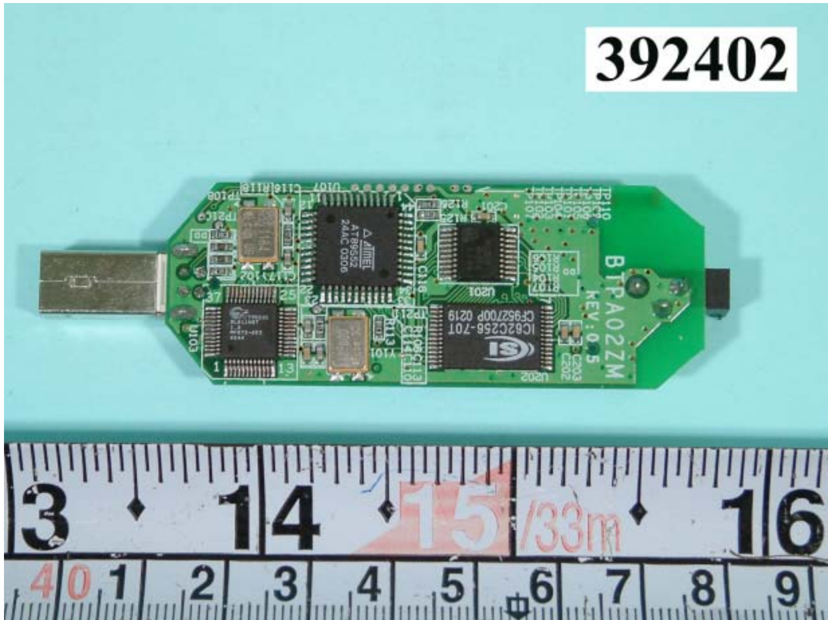
REAR SIDE MAIN BOARD
