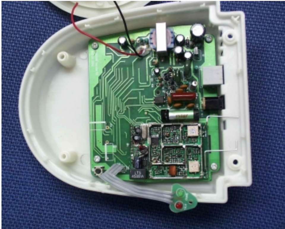
Base Main PCB comp side
