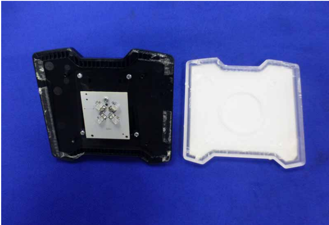
Figure 4 Inside of the UET
