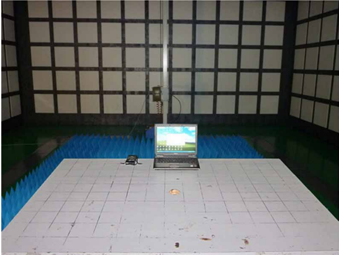
(At Anechoic 3m Chamber Test 1GHz -18GHz)
