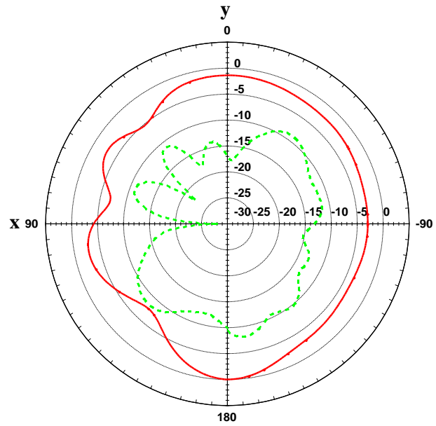
xy plane Etheta — Ephi - - - -
