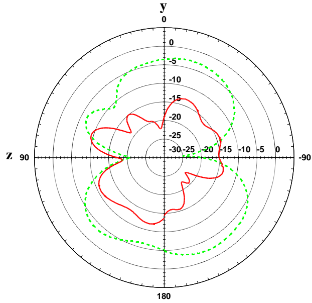
yz plane Etheta — Ephi - - - -
