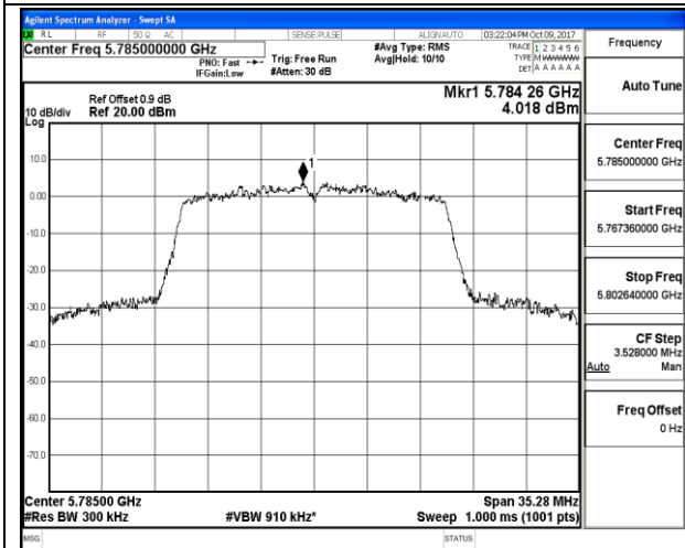
802.11a_Middle Channel / 5785MHz
