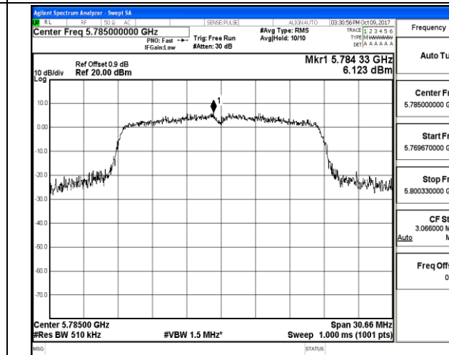
802.11n HT20_Middle Channel / 5785MHz
