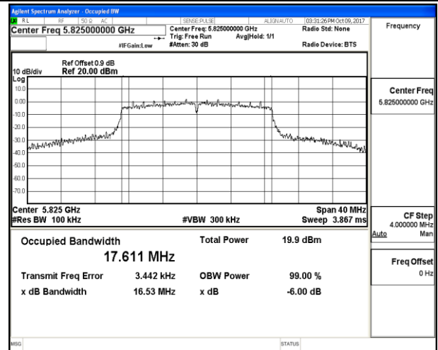
802.11n HT20_High Channel / 5825MHz
