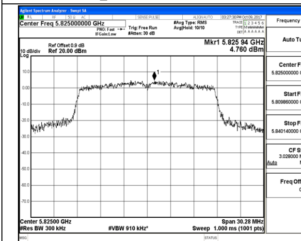
802.11a_High Channel / 5825MHz
