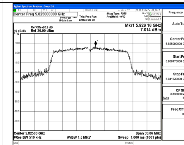
802.11n HT20_High Channel / 5825MHz
