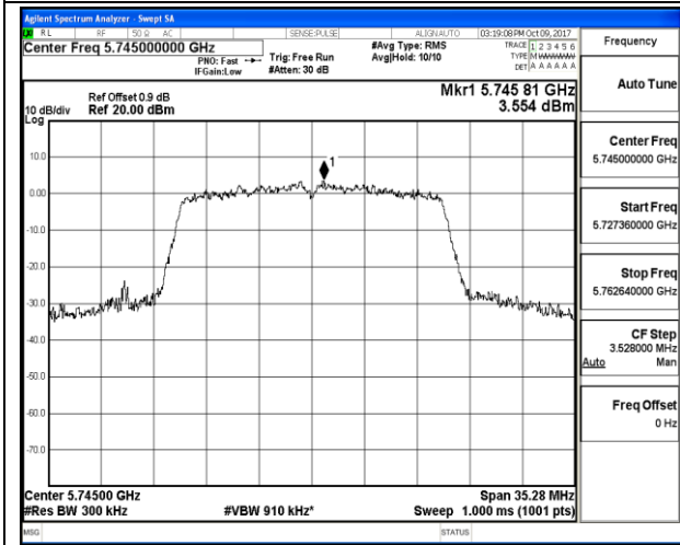
802.11a_Low Channel / 5745MHz
