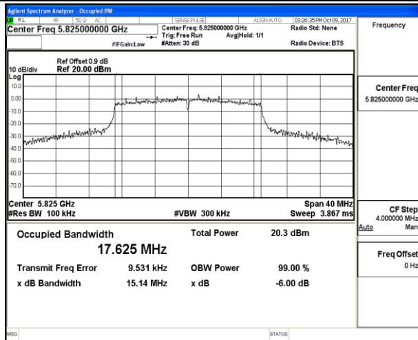
802.11a_High Channel / 5825MHz
