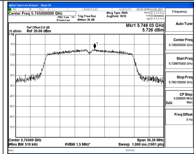
802.11n HT20_Low Channel / 5745MHz
