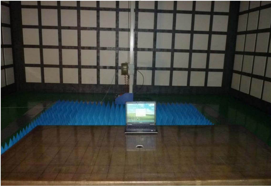
(At Anechoic 3m Chamber Test 1GHz -6GHz)
