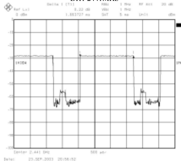
DH3 2441MHz
