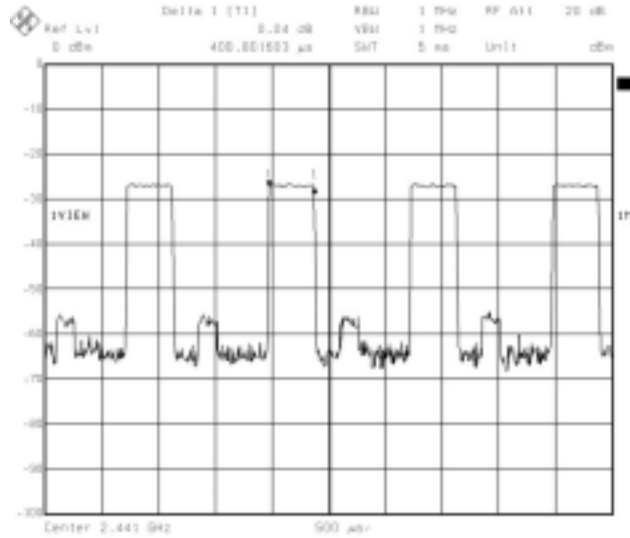
DH1 2441MHz
