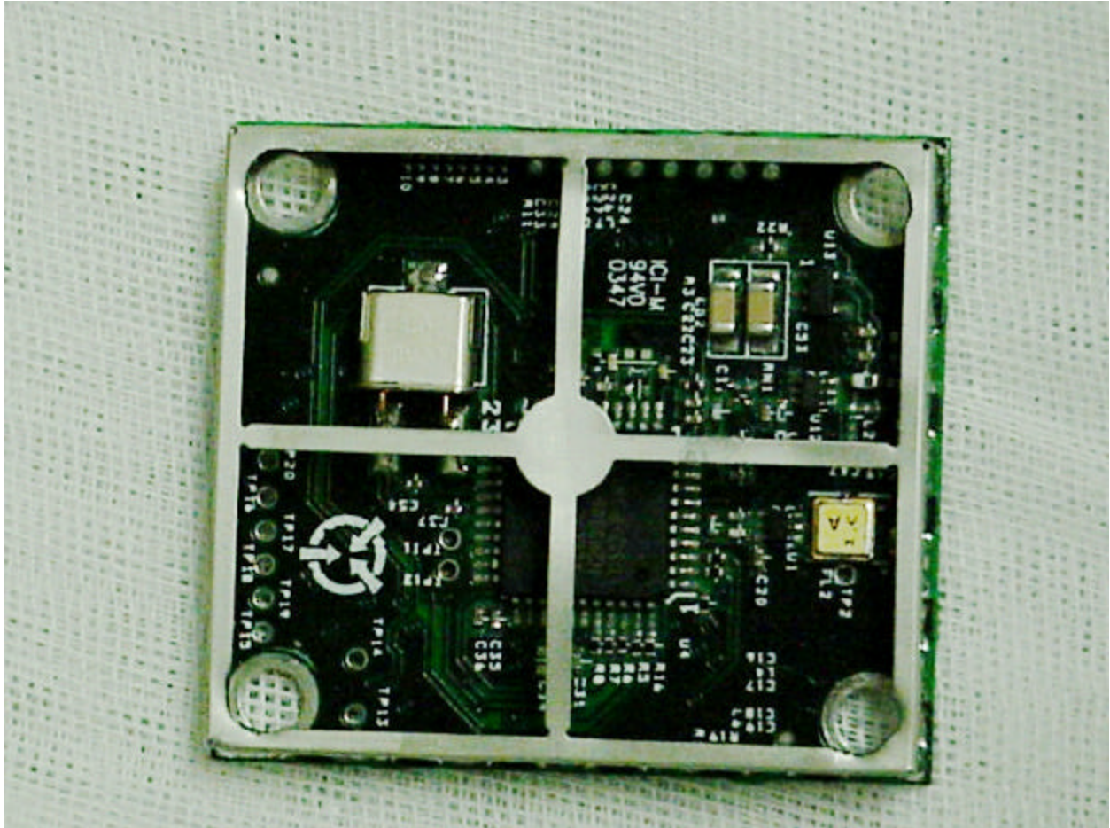
Photo 7. Transmitter Board, Top Side
