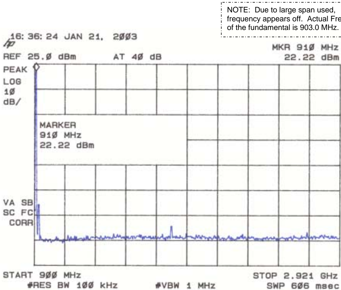
Figure 4b Antenna Conducted Spurious Emissions 5.247(c) Low
