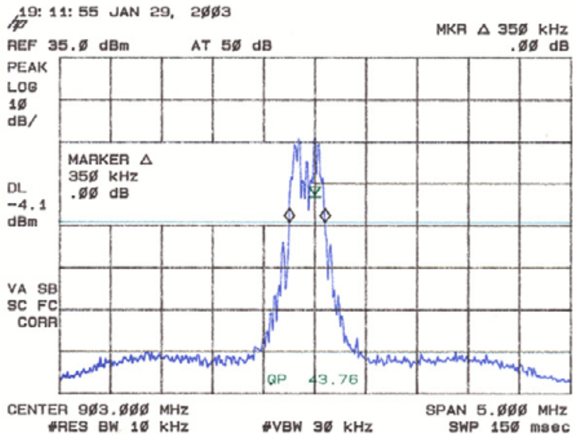
Figure 5a. 20 dB Bandwidth per FCC Section 15.247(a)(1)(i) (low)
