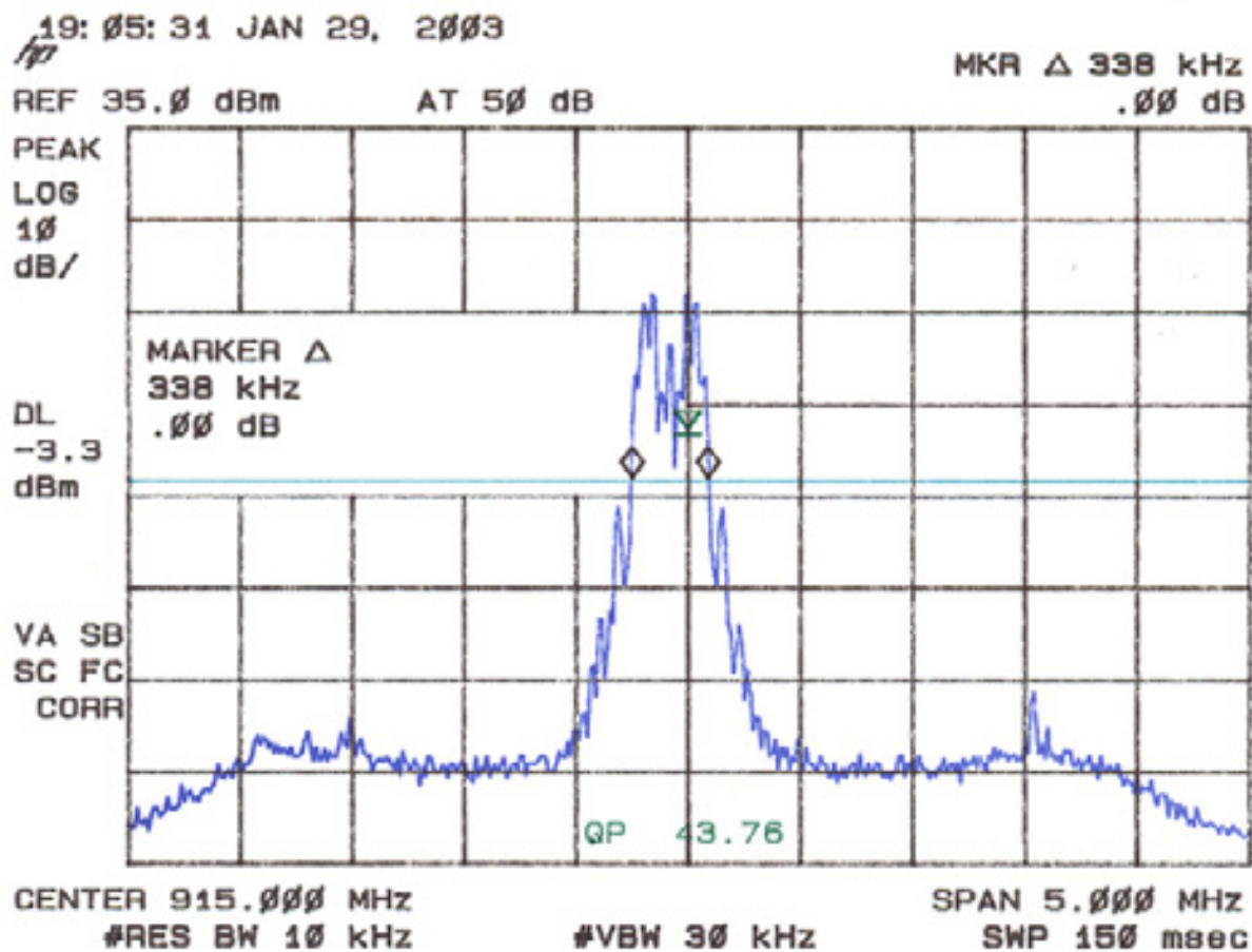
Figure 5b. 20 dB Bandwidth per FCC Section 15.247(a)(1)(i) (Mid)
