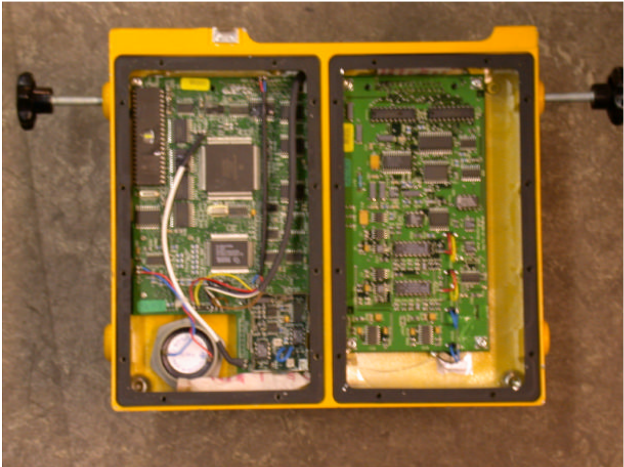
Figure 1. Back side of the CUII with hatches opened. The cpu-card is to the left and the timing board to the right
