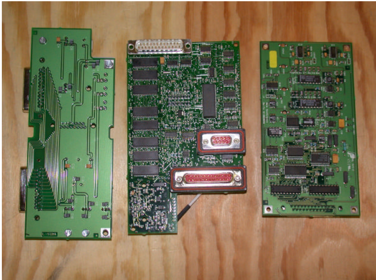
Figure 4. Back side of dc/dc-board, cpu-board and front site of timing board
