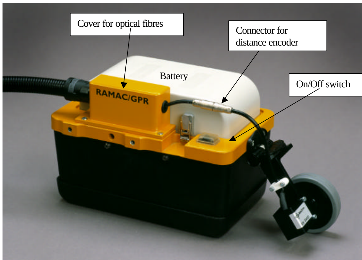
Picture 1. 1GHz unit with battery and distance encoder
