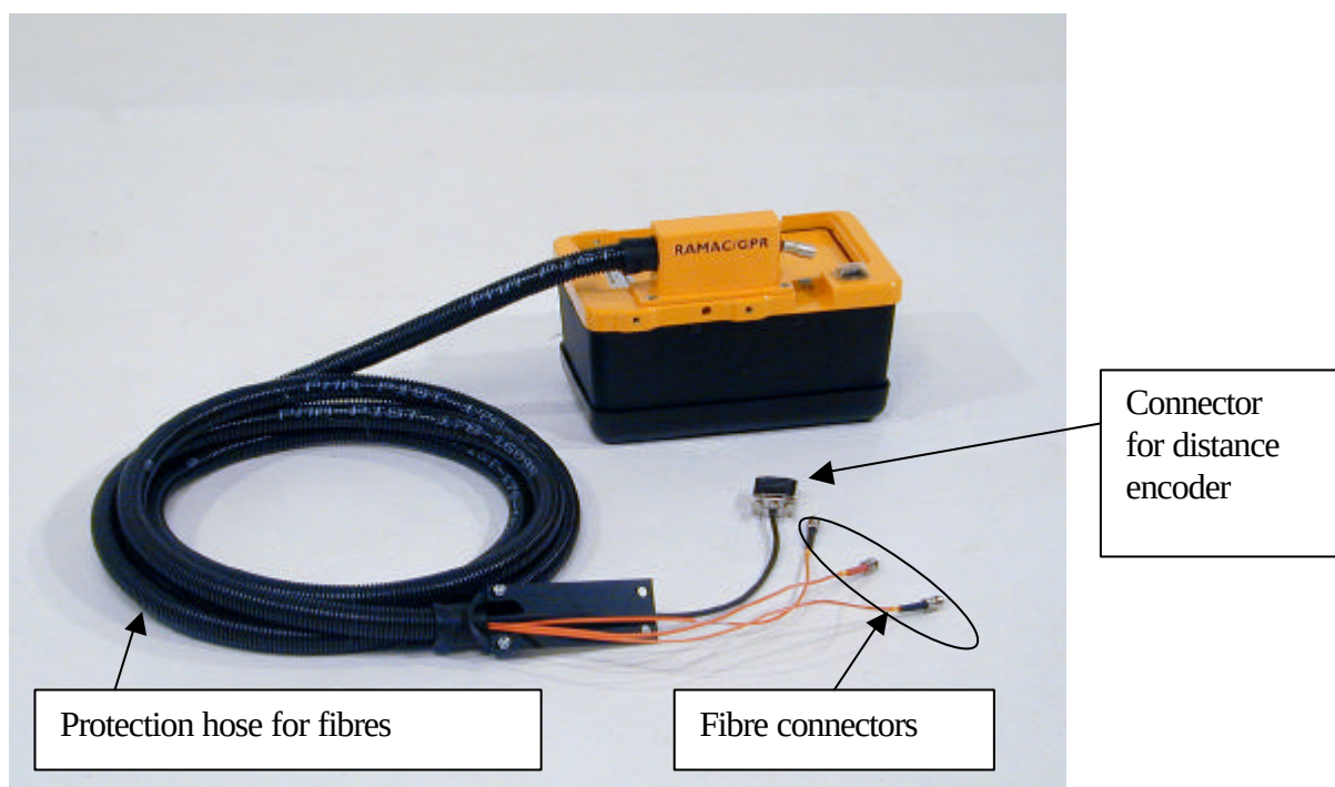
Picture 2. 1GHz with cable hose
