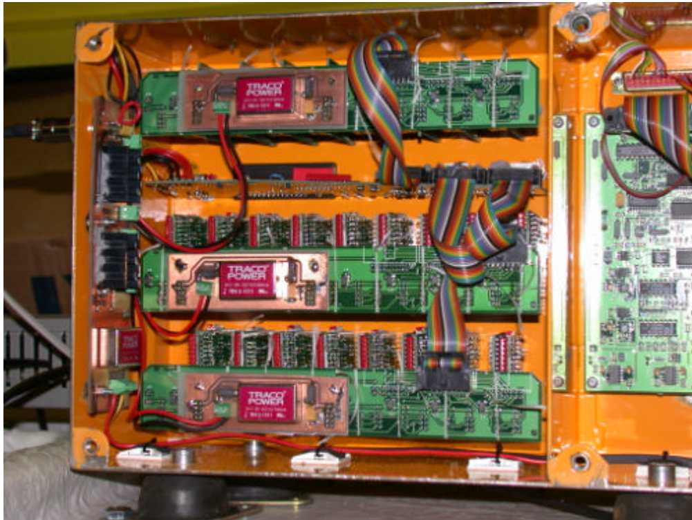
Control signal distribution section
