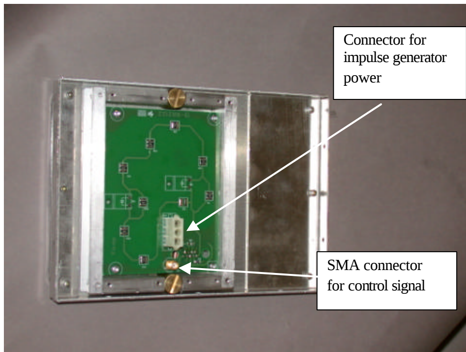
Inside antenna top with current limiting resistors and connectors to impulse generator.
