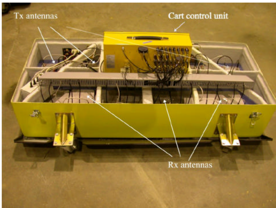
Overview over interior of Cart400
