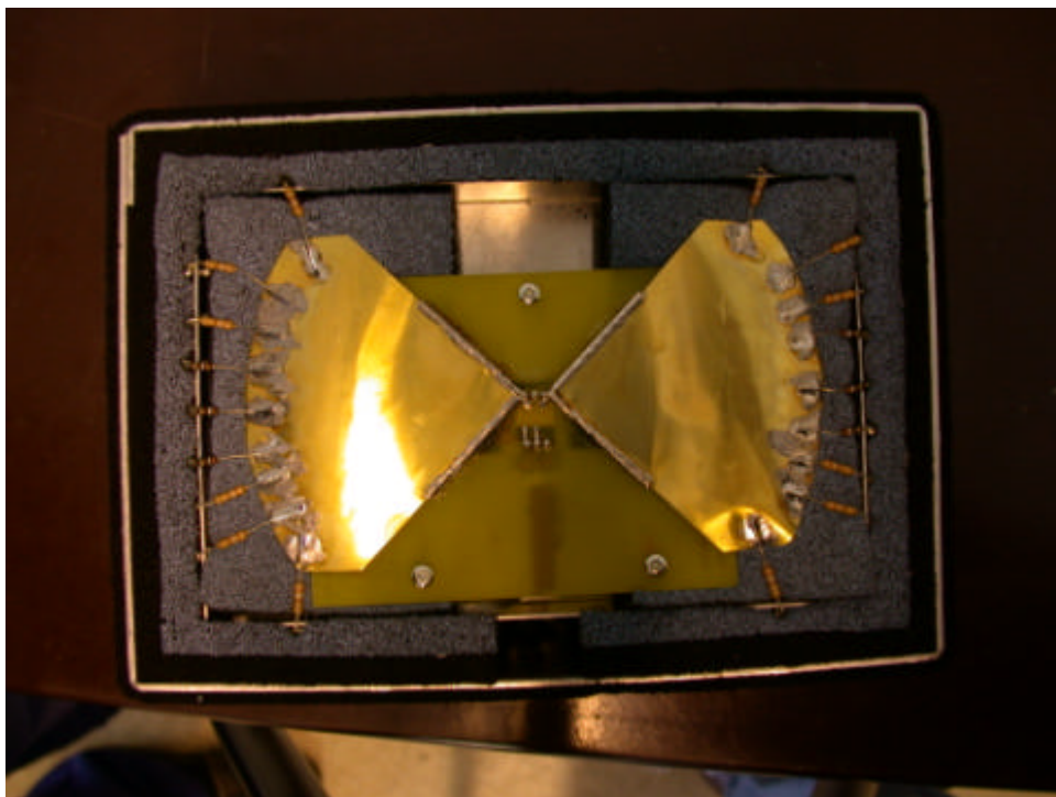
Tx antenna complete, bottom view. Showing antenna flares and loading resistors.
