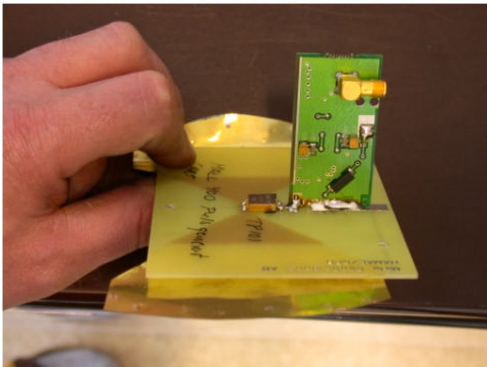
Impulse generator, balun and antenna. Back side
