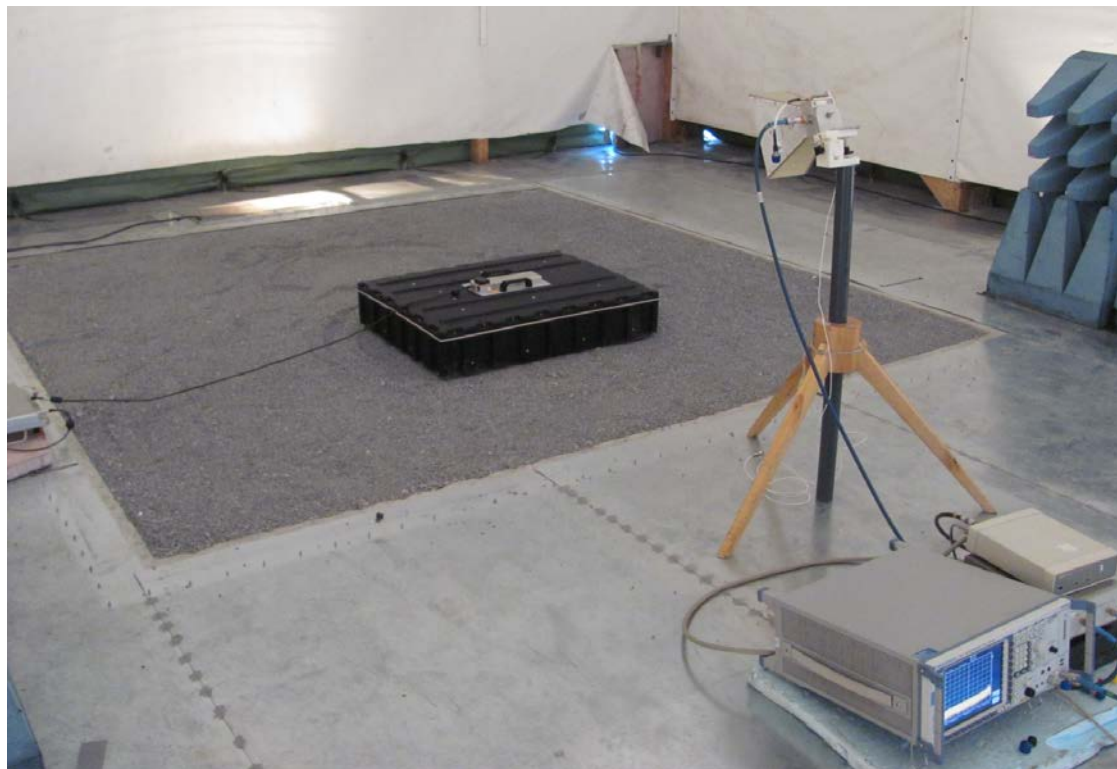
Measurements with horn-receiver.
