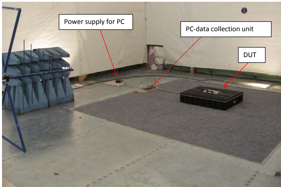
Test setup photos - 80MHZHDR
