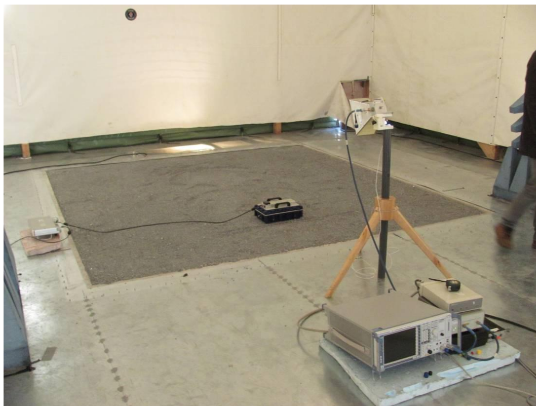
Picture 4. Measurement setup.
