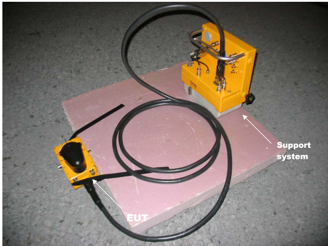
Picture 1: EUT set-up on sand bed
